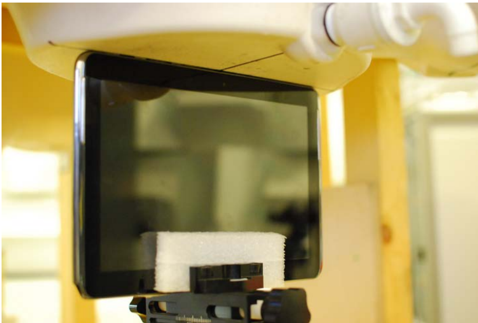
SAR Test Setup Photo 2: Top at 0.0 cm
