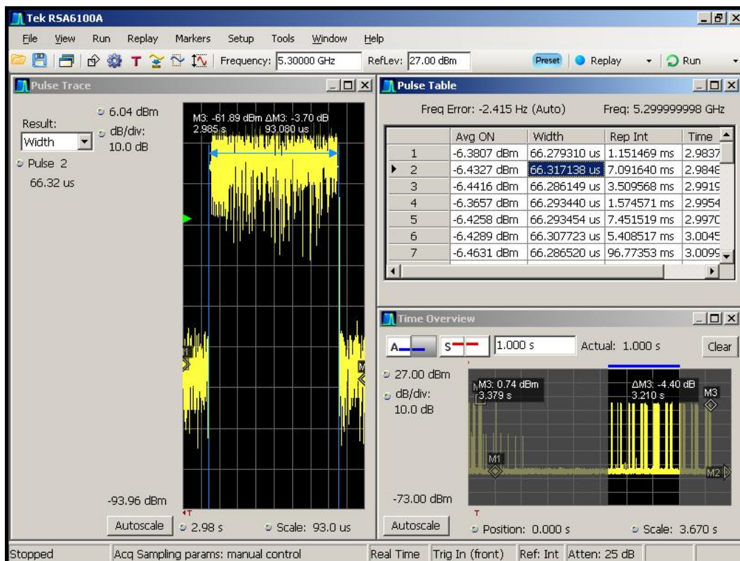
Figure 5-6. Pulse width analysis using Pulse Table and Pulse Trace Function
