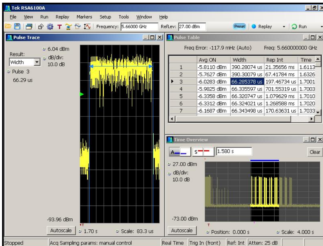
Figure 6-6. Pulse width analysis using Pulse Table and Pulse Trace Function
