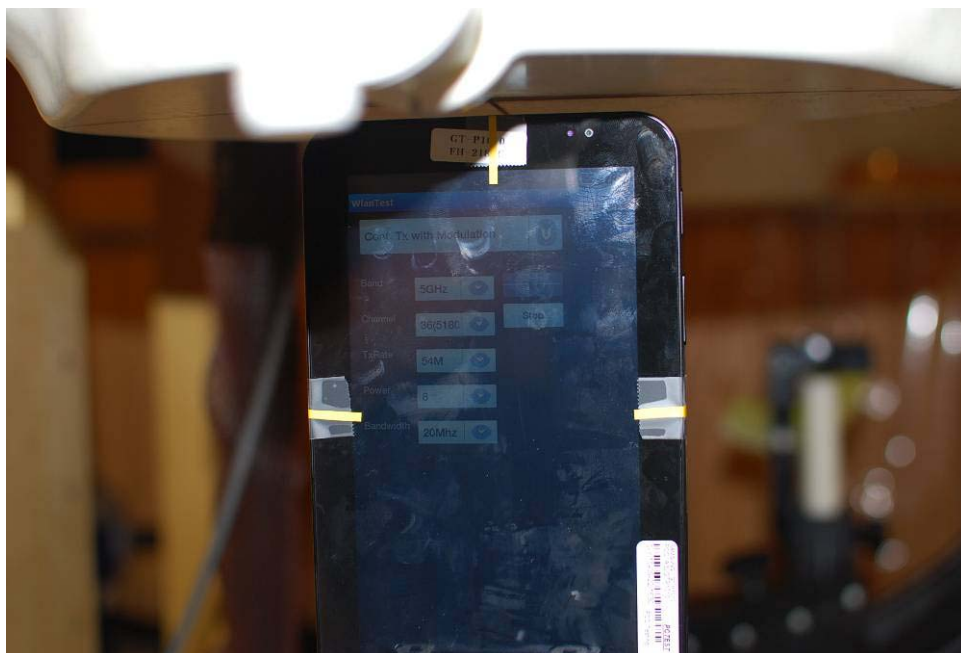
Figure 17-2 SAR Test Setup Photo 2 – Top Edge
