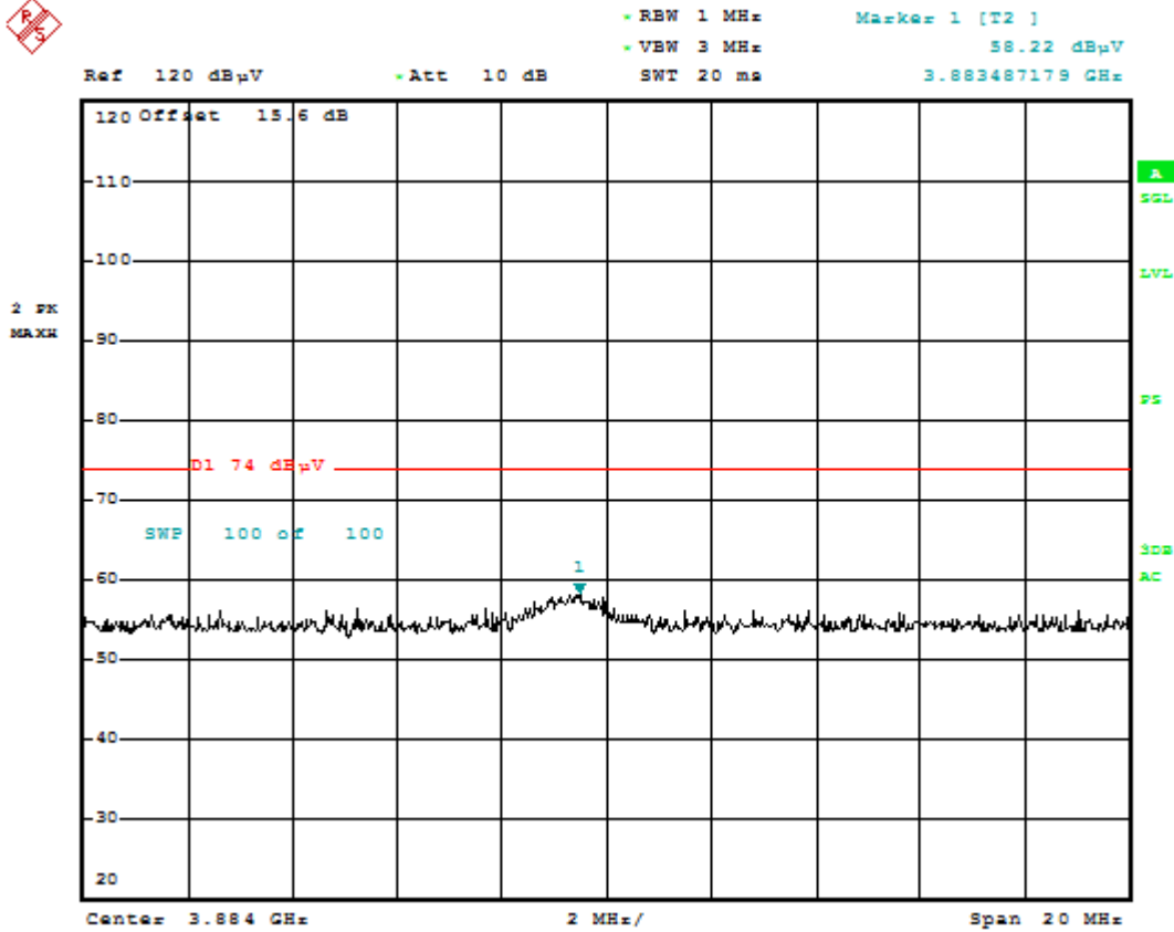
Plot 6-64. Radiated Spurious Plot Peak Measurement (802.11a – Ch. 165)
