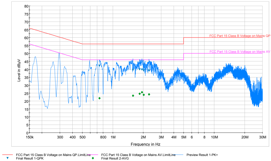
Plot 6-72. Line Conducted Plot with 802.11a (N)
