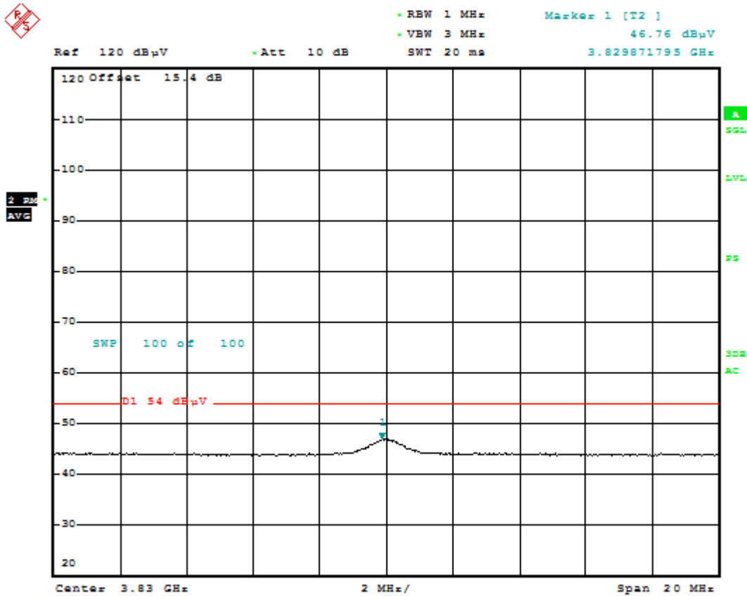
Plot 6-59. Radiated Spurious Plot Average Measurement (802.11a – Ch. 149)
