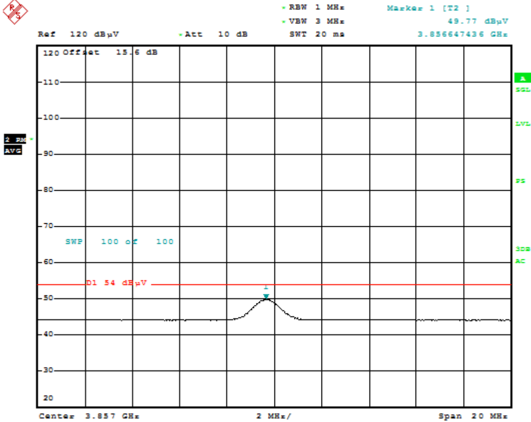
Plot 6-61. Radiated Spurious Plot Average Measurement (802.11a – Ch. 157)
