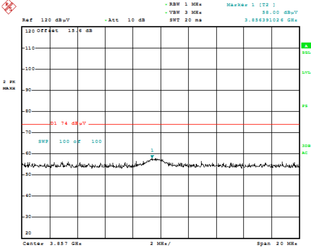
Plot 6-62. Radiated Spurious Plot Peak Measurement (802.11a – Ch. 157)
