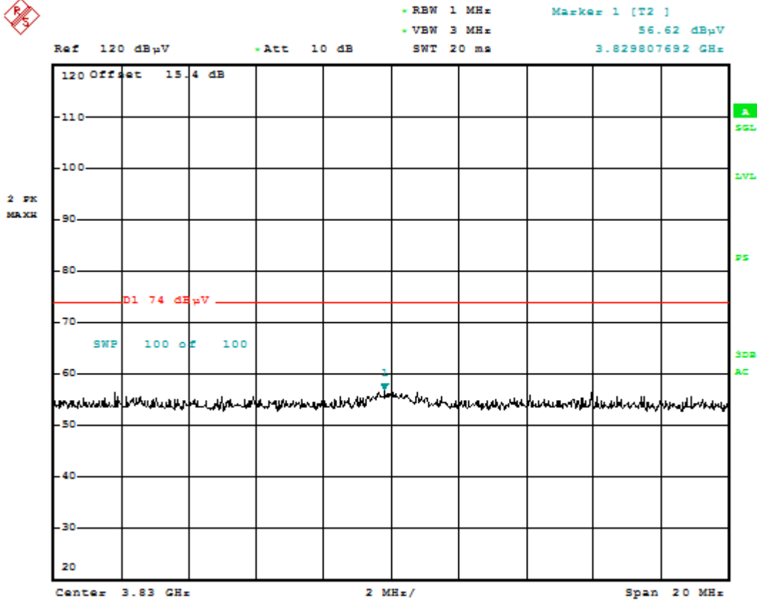
Plot 6-60. Radiated Spurious Plot Peak Measurement (802.11a – Ch. 149)
