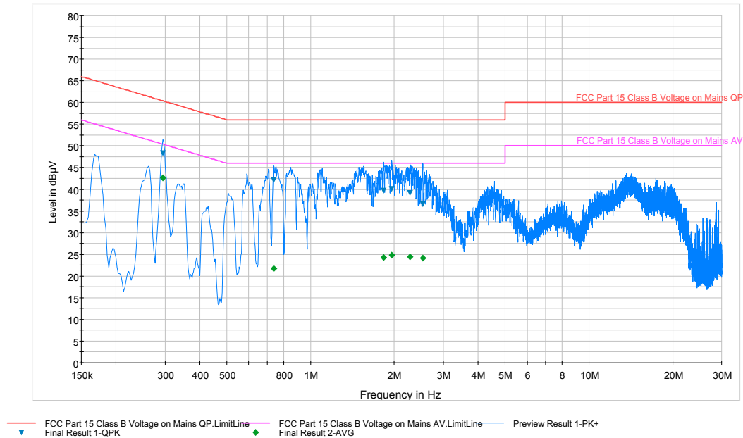
Plot 6-70. Line Conducted Plot with 802.11b (N)
