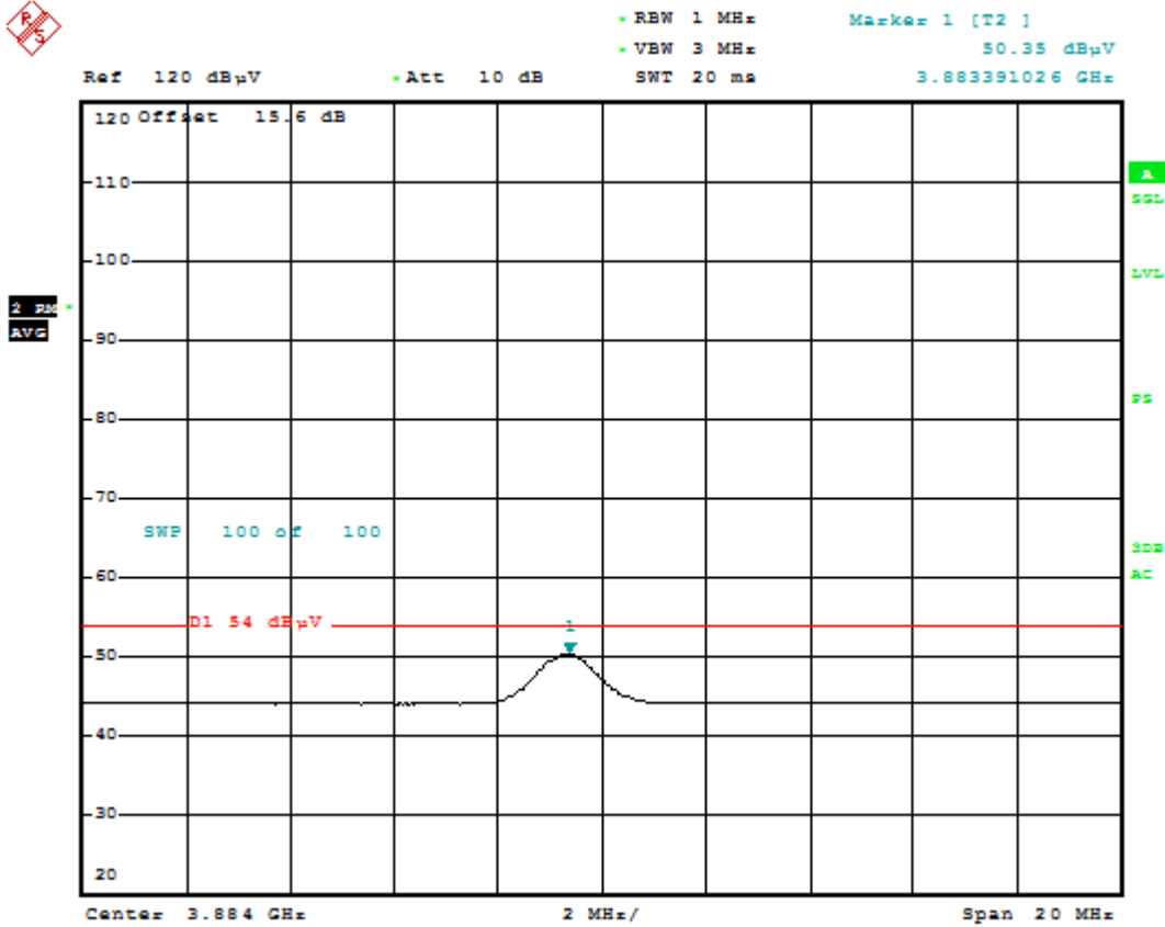
Plot 6-63. Radiated Spurious Plot Average Measurement (802.11a – Ch. 165)
