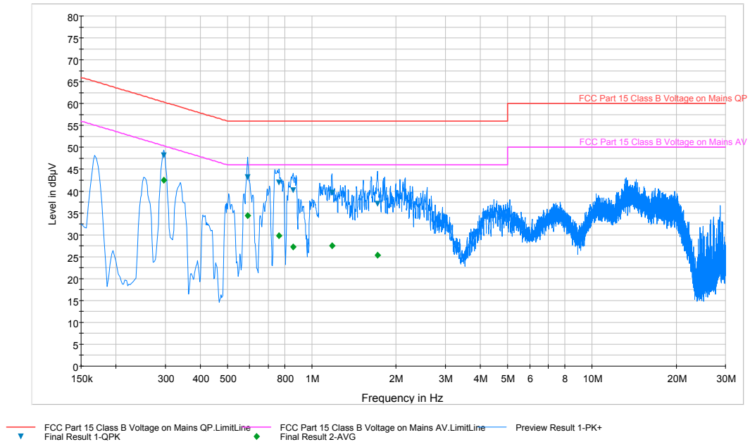
Plot 6-69. Line Conducted Plot with 802.11b (L1)
