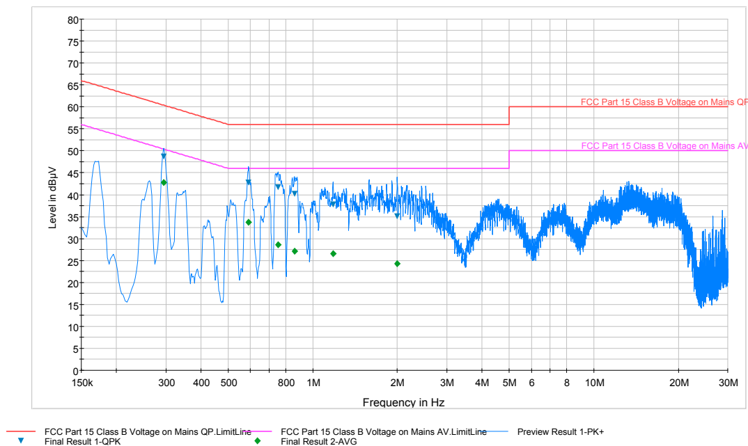
Plot 6-71. Line Conducted Plot with 802.11a (L1)
