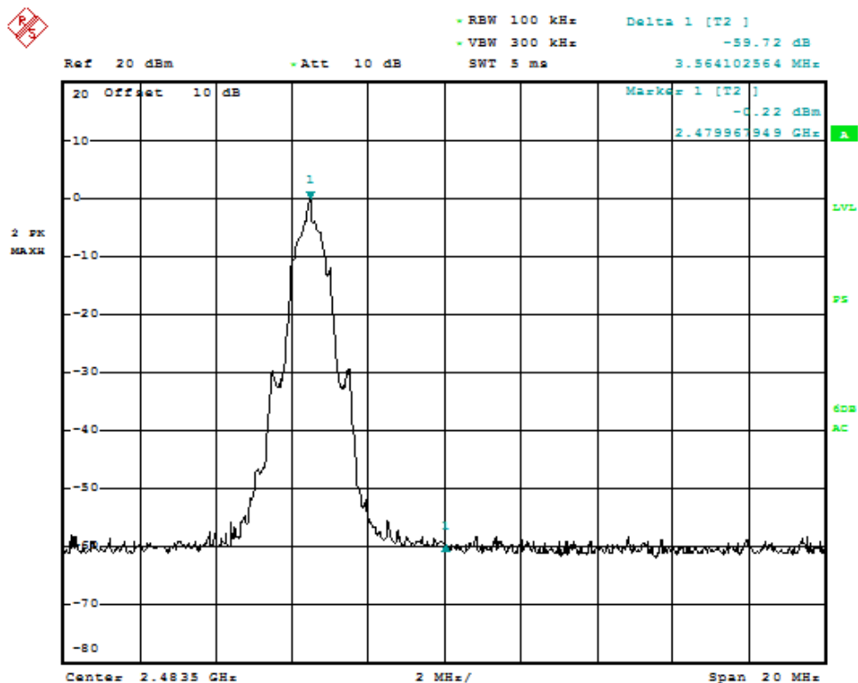
Plot 6-18. Measurement of Delta from Fundamental to Band Edge (Ch. 78)
