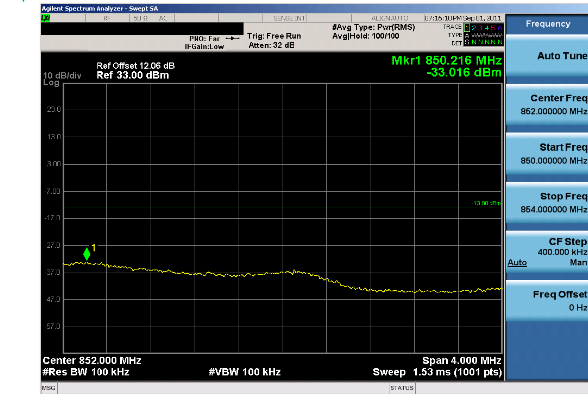
Plot 7-33. 4MHz Span Plot (Cellular WCDMA Mode – Ch. 4233)
