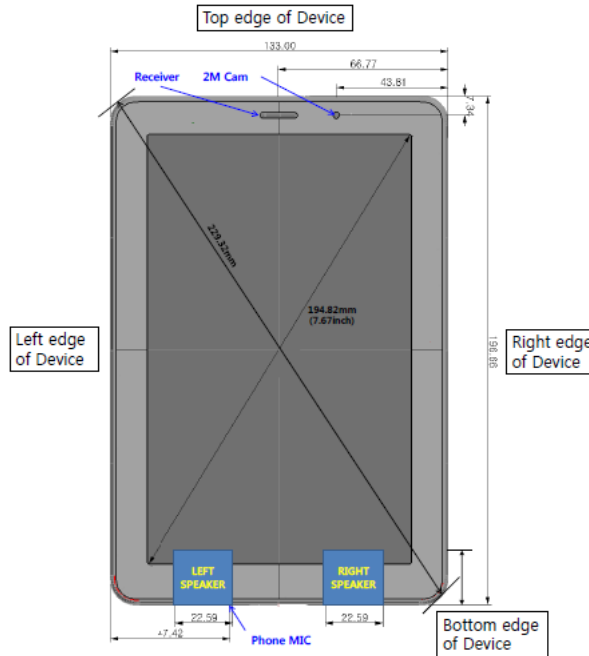
Figure 11-1 Front View of Device
