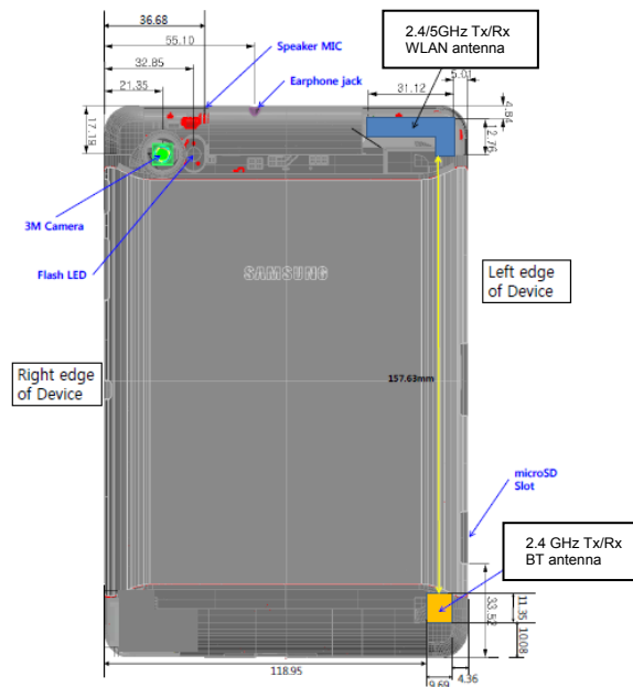
Figure 11-2 Back View of Device
