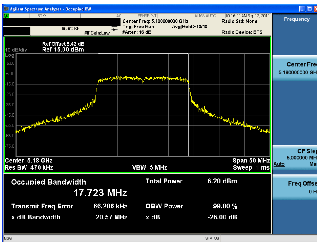
Plot 6-4. 26dB Bandwidth Plot (802.11n (UNII Band 1) – Ch. 36)
