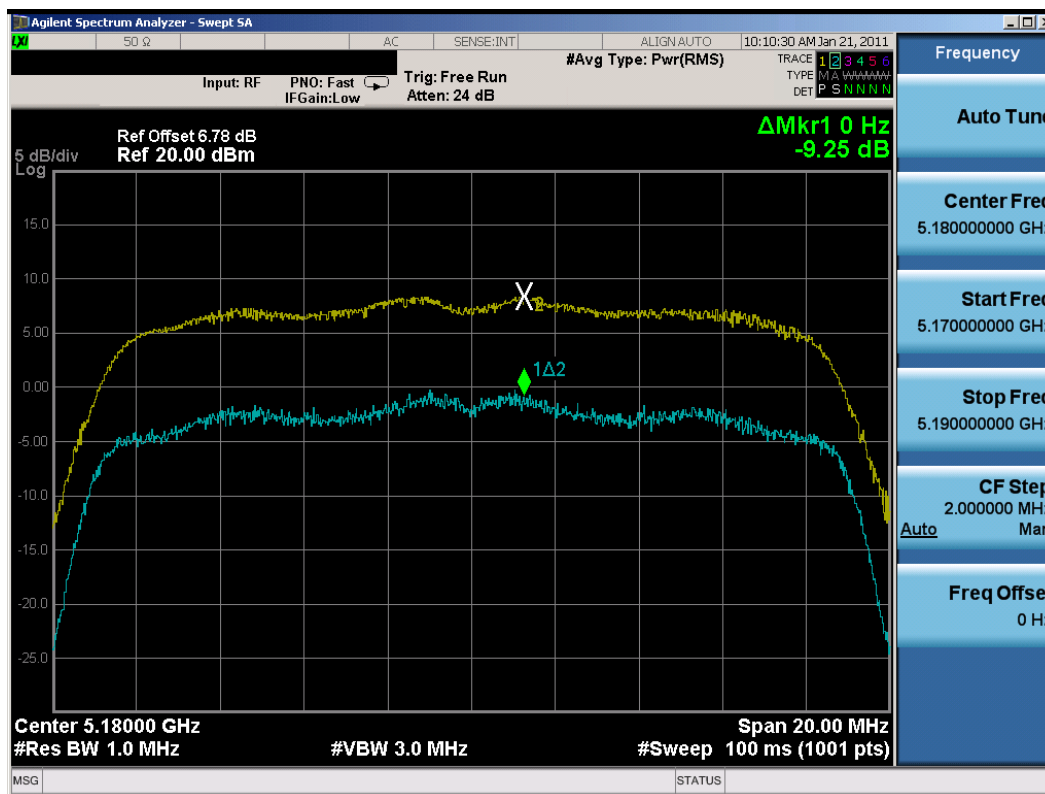
Plot 6-40. Peak Excursion Ratio Plot (802.11n (UNII) – Ch. 36)
