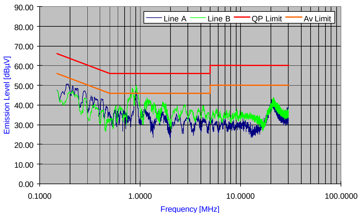
Plot 6-55. Line Conducted Plot with 802.11a (UNII-I Band)
