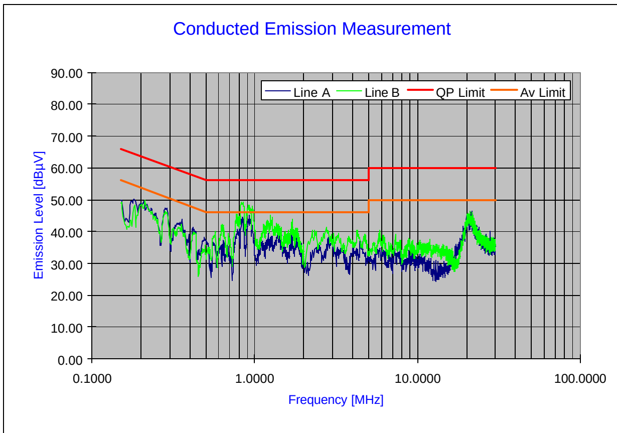
Plot 6-60. Line Conducted Plot with 802.11n (UNII-III Band)
