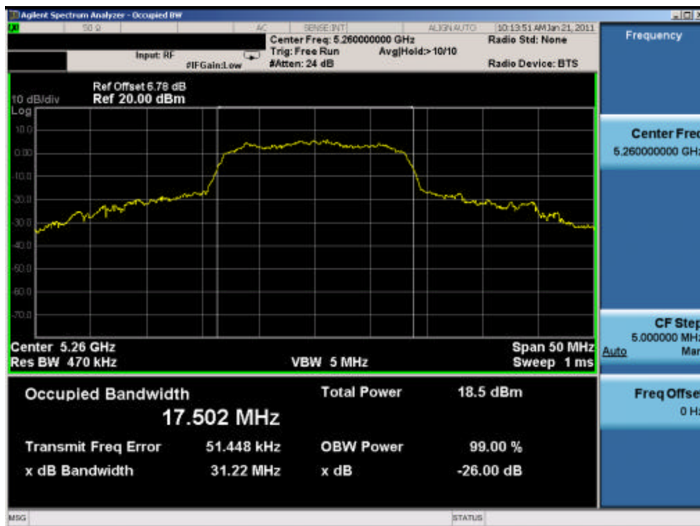
Plot 6-7. 26dB Bandwidth Plot (802.11a (UNII) – Ch. 52)
