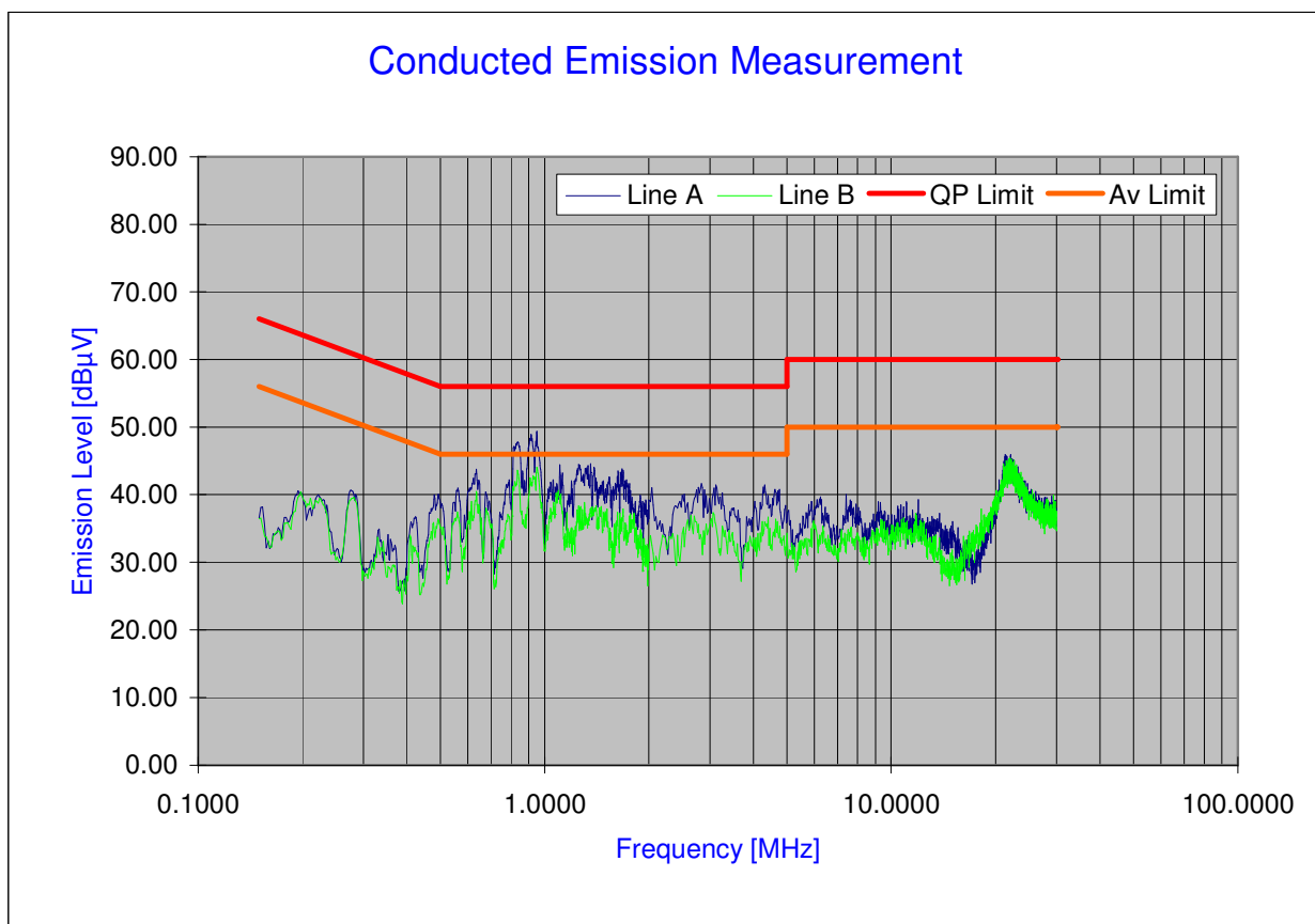
Plot 6-55. Line Conducted Plot with 802.11a
