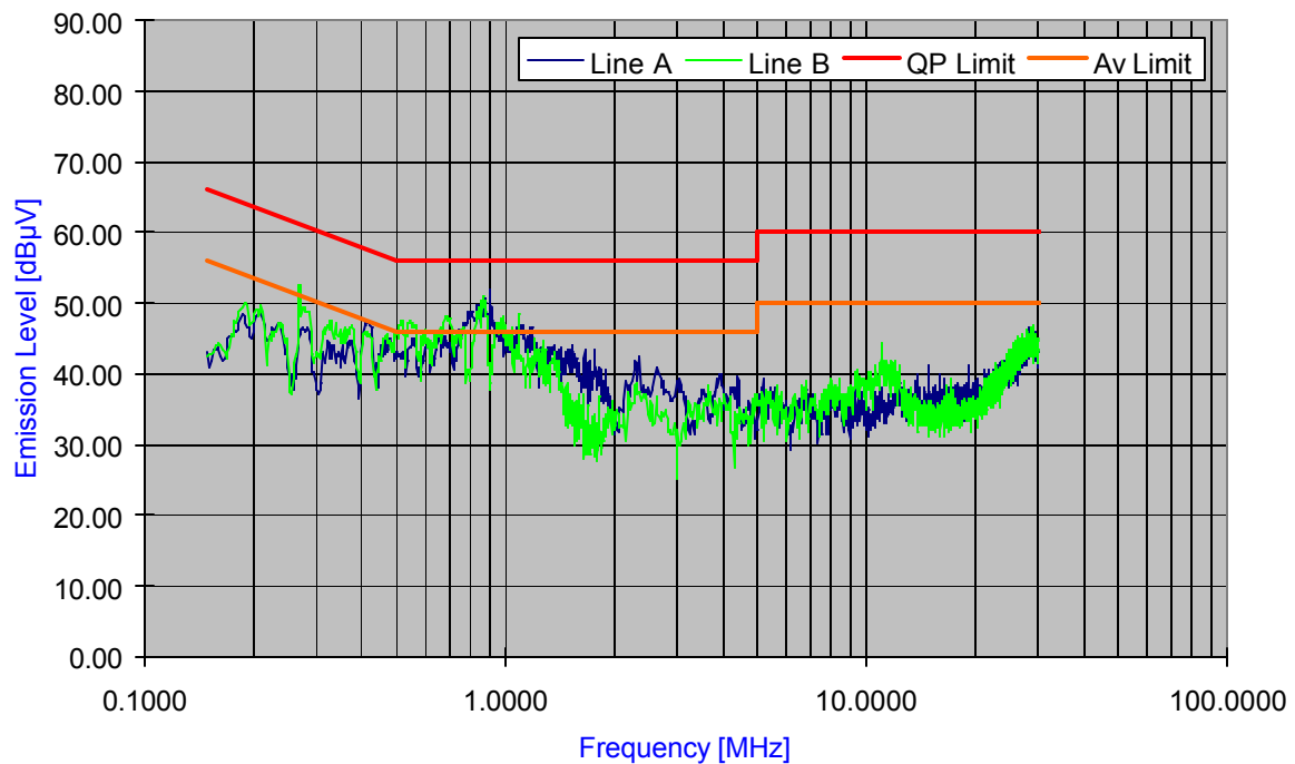
Plot 6-57. Line Conducted Plot with 802.11n (5.8GHz)
