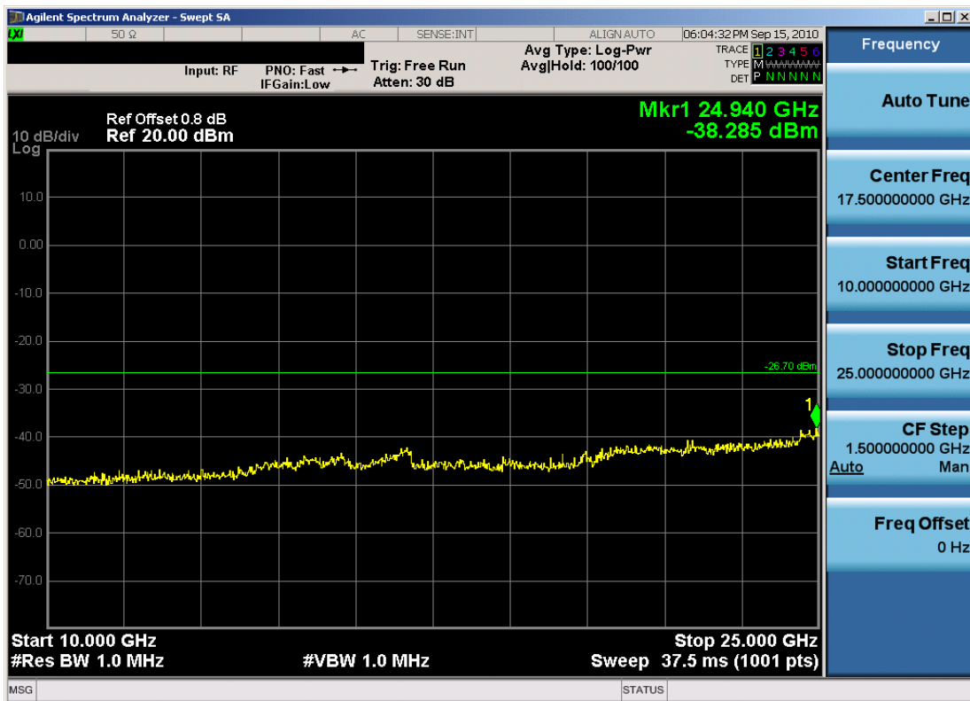
Plot 6-16. Conducted Spurious Plot (802.11b – Ch. 11)
