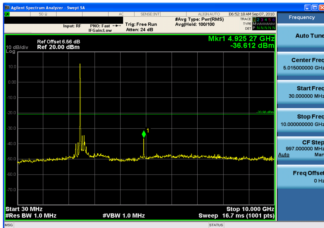
Plot 6-17. Conducted Spurious Plot (802.11b – Ch. 11)
