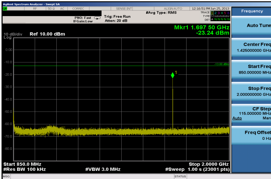
Plot 6-11. Conducted Spurious Plot (Cellular GSM Mode – Ch. 251)
