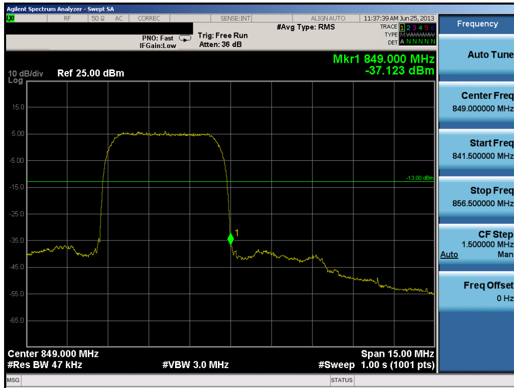
Plot 6-30. Band Edge Plot (Cellular WCDMA Mode – Ch. 4233)
