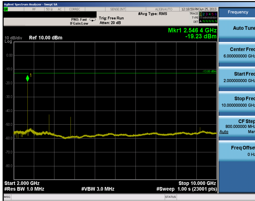
Plot 6-12. Conducted Spurious Plot (Cellular GSM Mode – Ch. 251)
