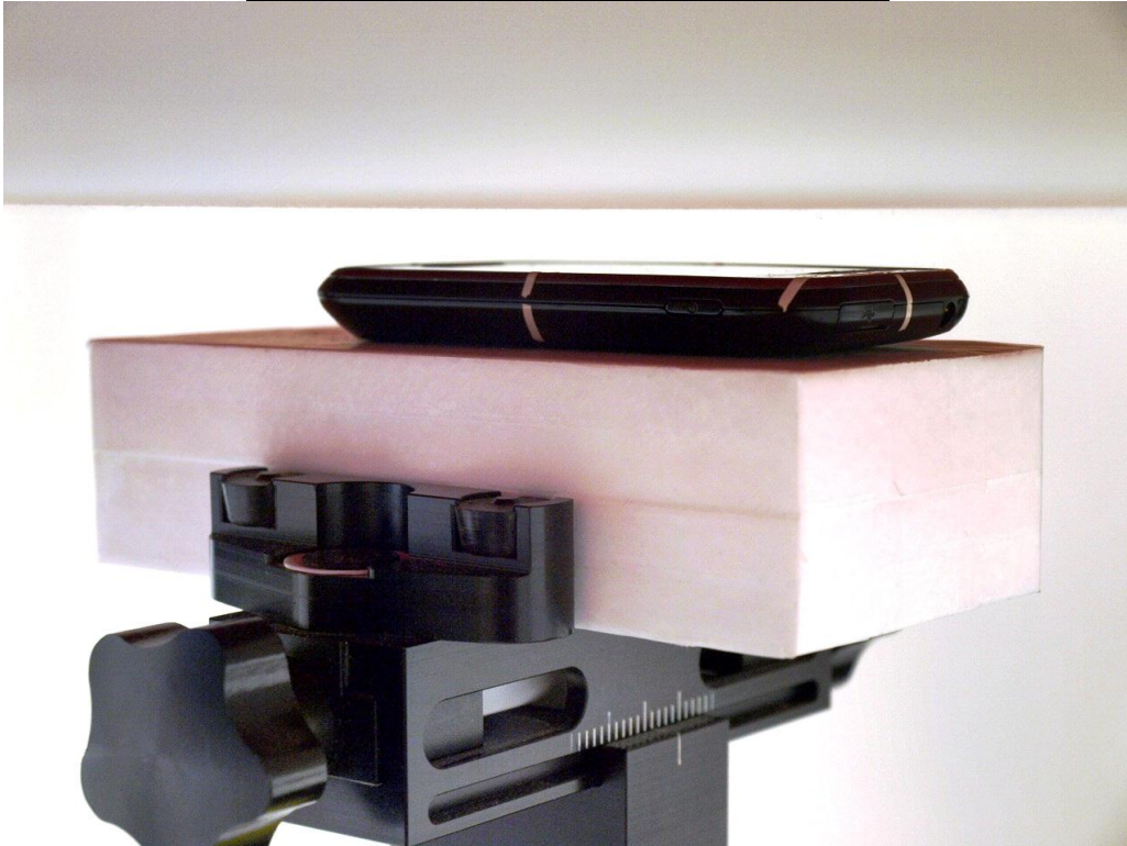
Body & Hotspot - Front w/ 10 mm Separation
