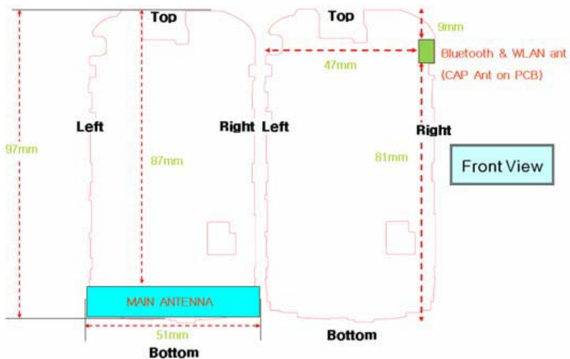
Figure 5.7 Identification of Sides for SAR Testing
