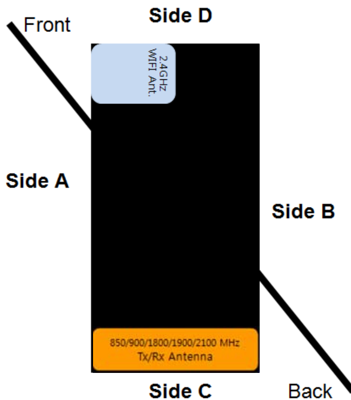
Figure 5.7 Identification of Sides for SAR Testing
