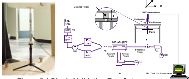
Figure 7.1 Dipole Validation Test Setup
