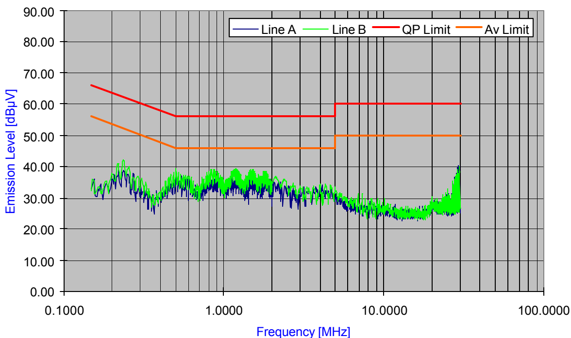
Plot 6-33. Line Conducted Plot with 802.11n
