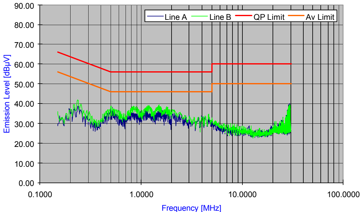
Plot 6-31. Line Conducted Plot with 802.11b
