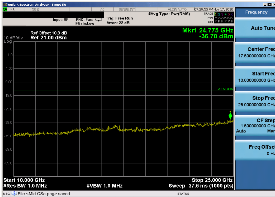
Plot 6-28. Conducted Spurious Plot (802.11b – Ch. 6)
