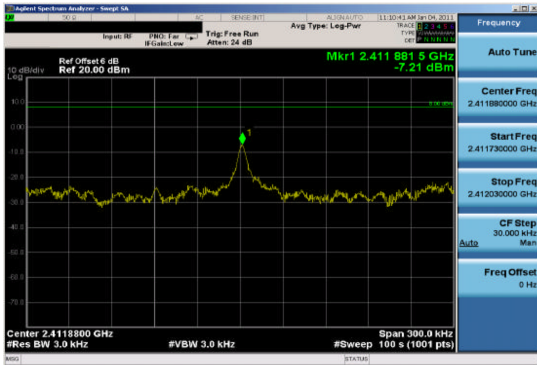
Plot 6-13. Power Spectral Density Plot (802.11g - Ch. 1)
