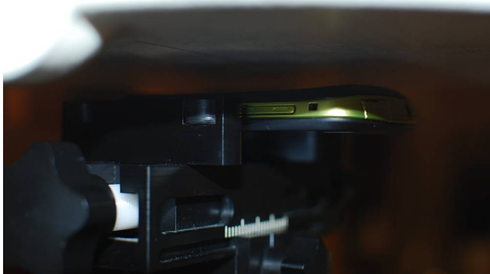
Figure 21-5 SAR Test Setup Photo 5: Back
