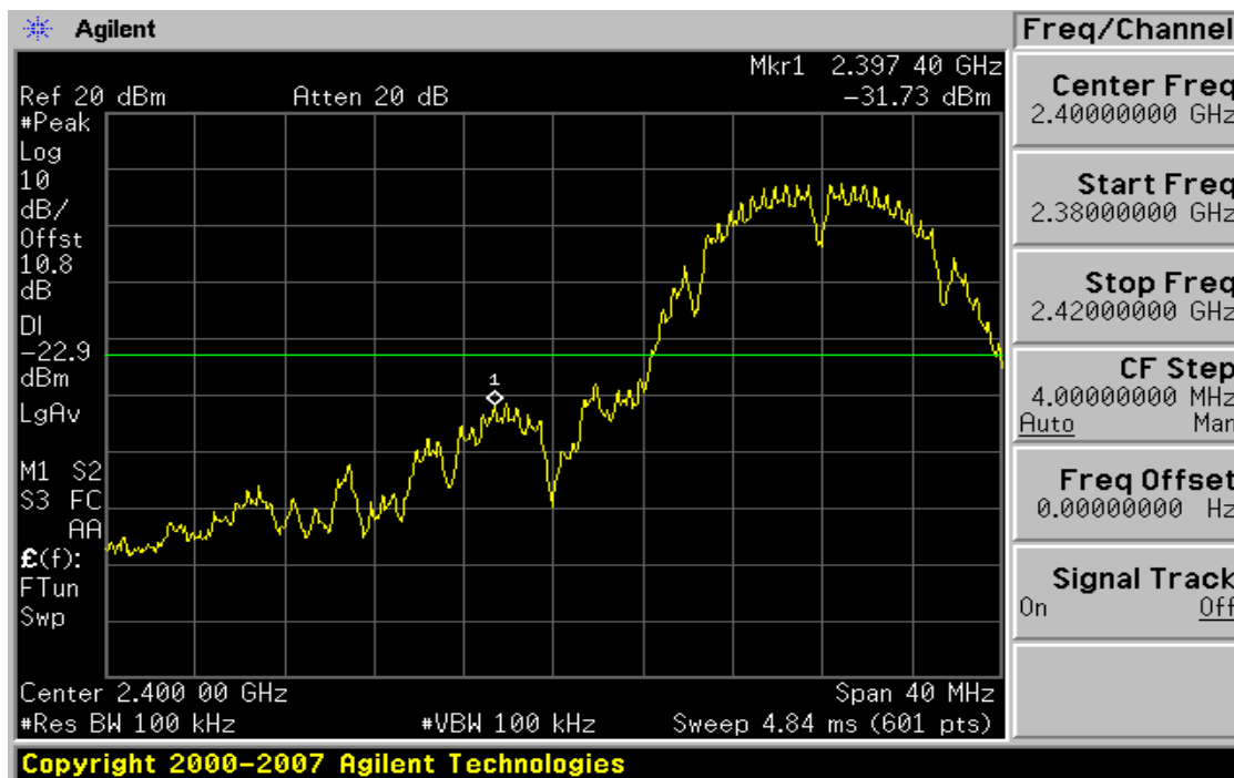
Plot 6-13. Band Edge Plot (802.11b – Ch. 1)
