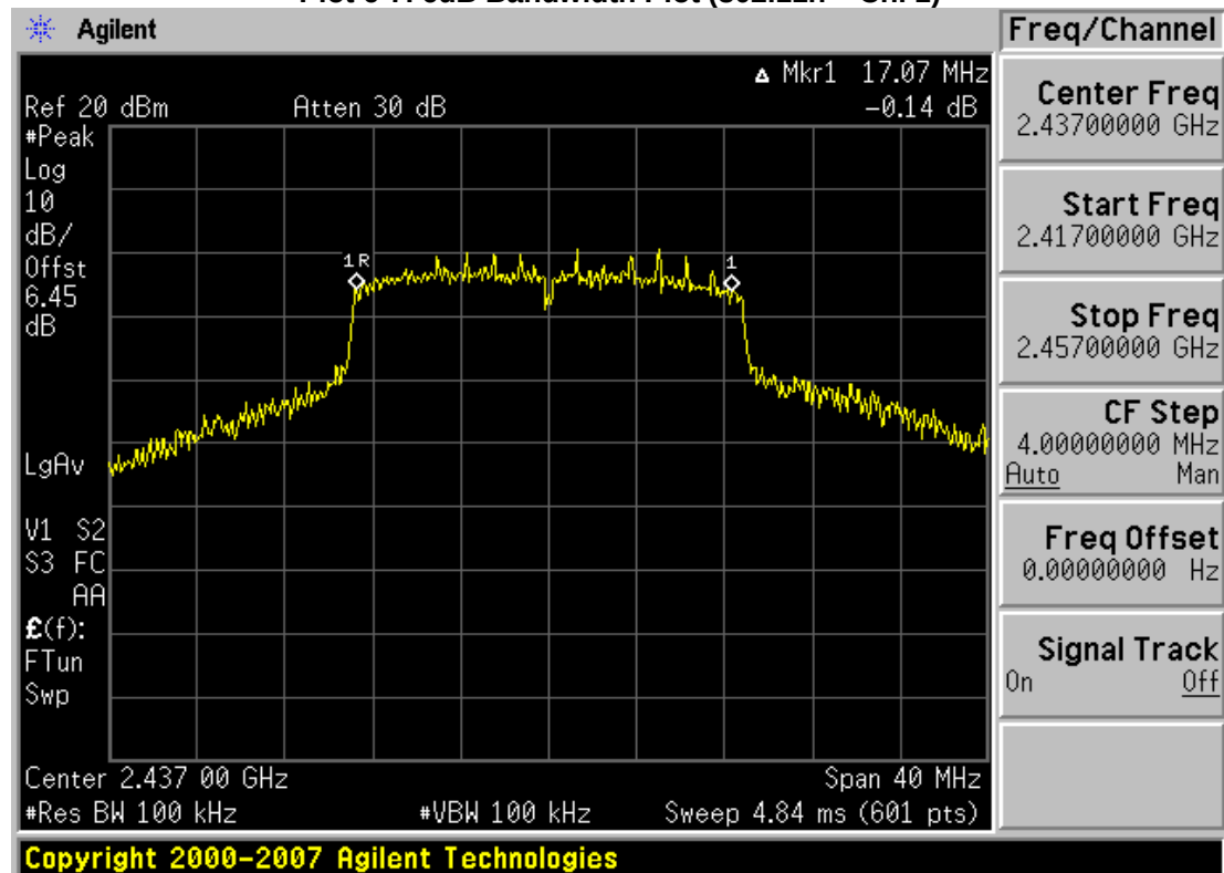
Plot 6-8. 6dB Bandwidth Plot (802.11n – Ch. 6)
