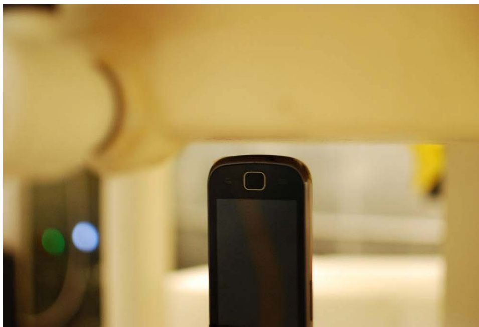
Figure 21-10 SAR Test Setup Photo 10 – Bottom at 1.0 cm
