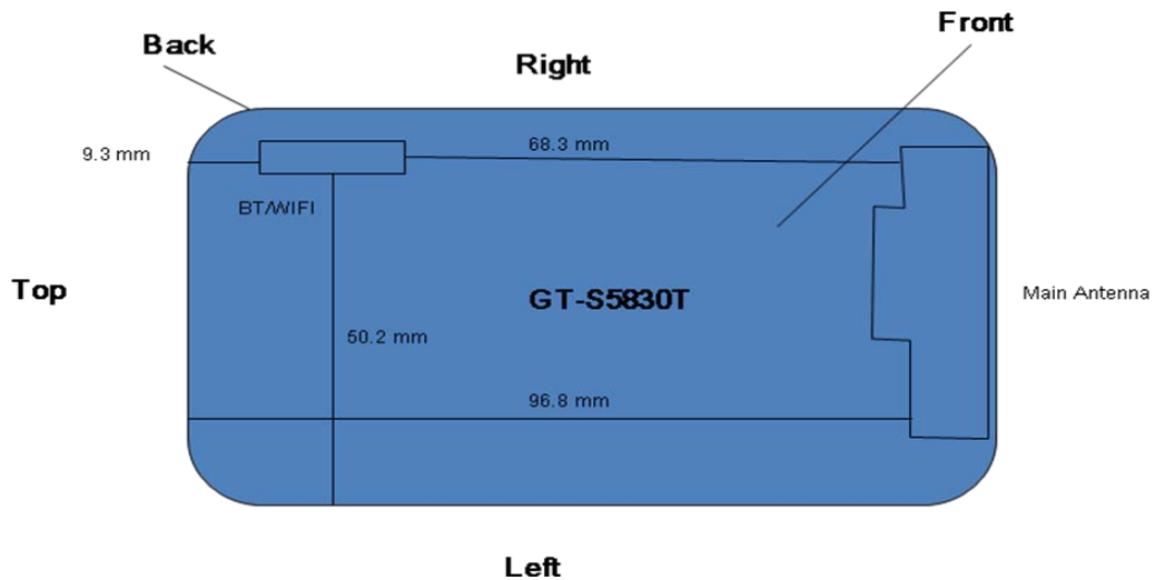
Figure 13-1 Identification of Sides for SAR Testing
