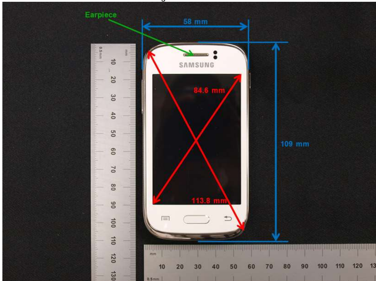
Diagonal Dimensions
