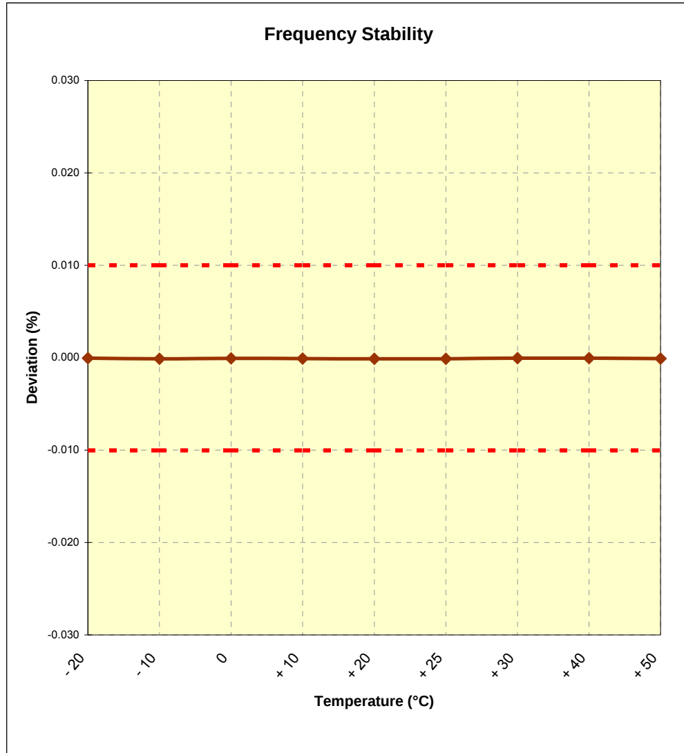
Figure 8-3. Frequency Stability Plot
