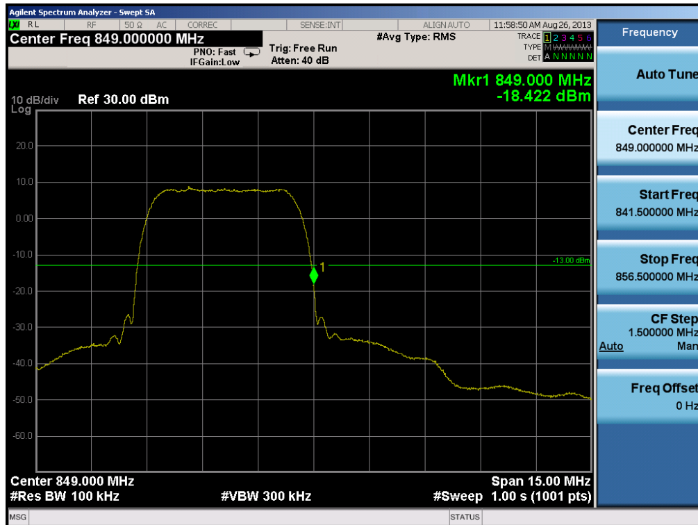
Plot 6-37. Band Edge Plot (Cellular WCDMA Mode – Ch. 4233)
