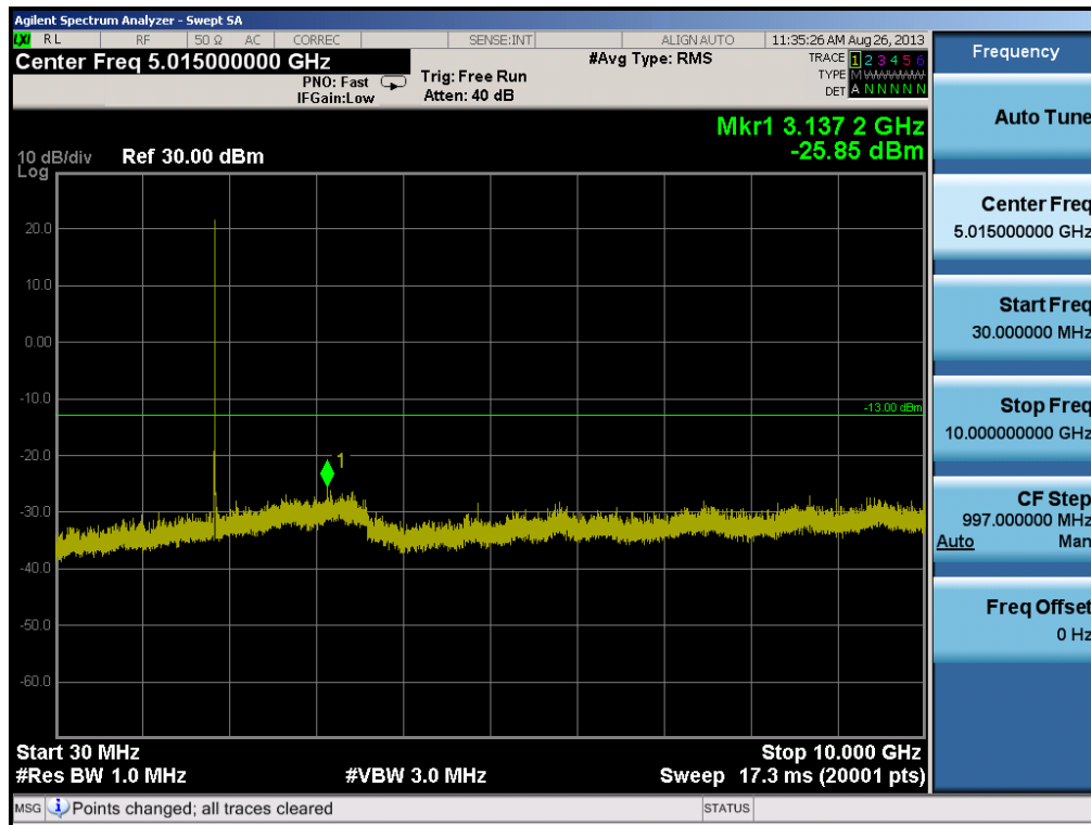
Plot 6-26. Conducted Spurious Plot (PCS WCDMA Mode – Ch. 9262)
