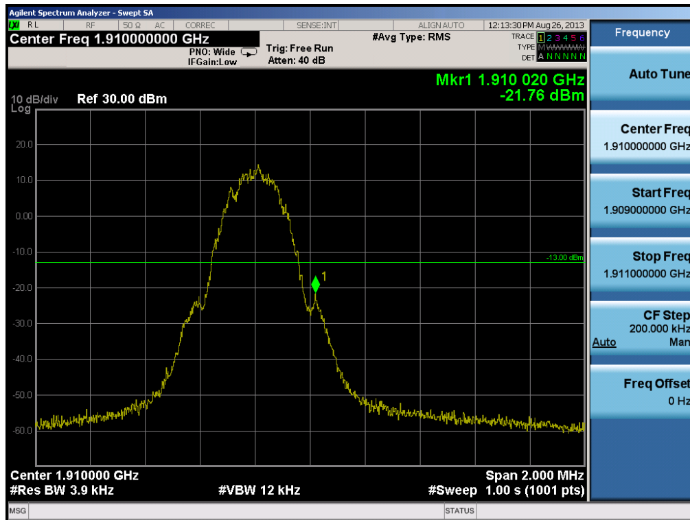
Plot 6-35. Band Edge Plot (PCS GSM Mode – Ch. 810)
