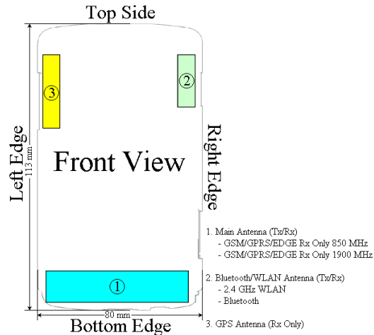
Figure 1-1 DUT Antenna Locations
