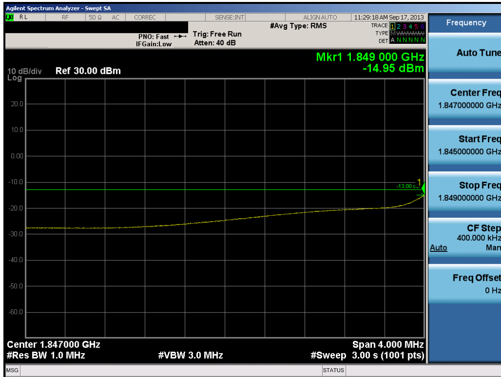
6-41. 4MHz Span Plot (PCS WCDMA Mode – Ch. 9262)
