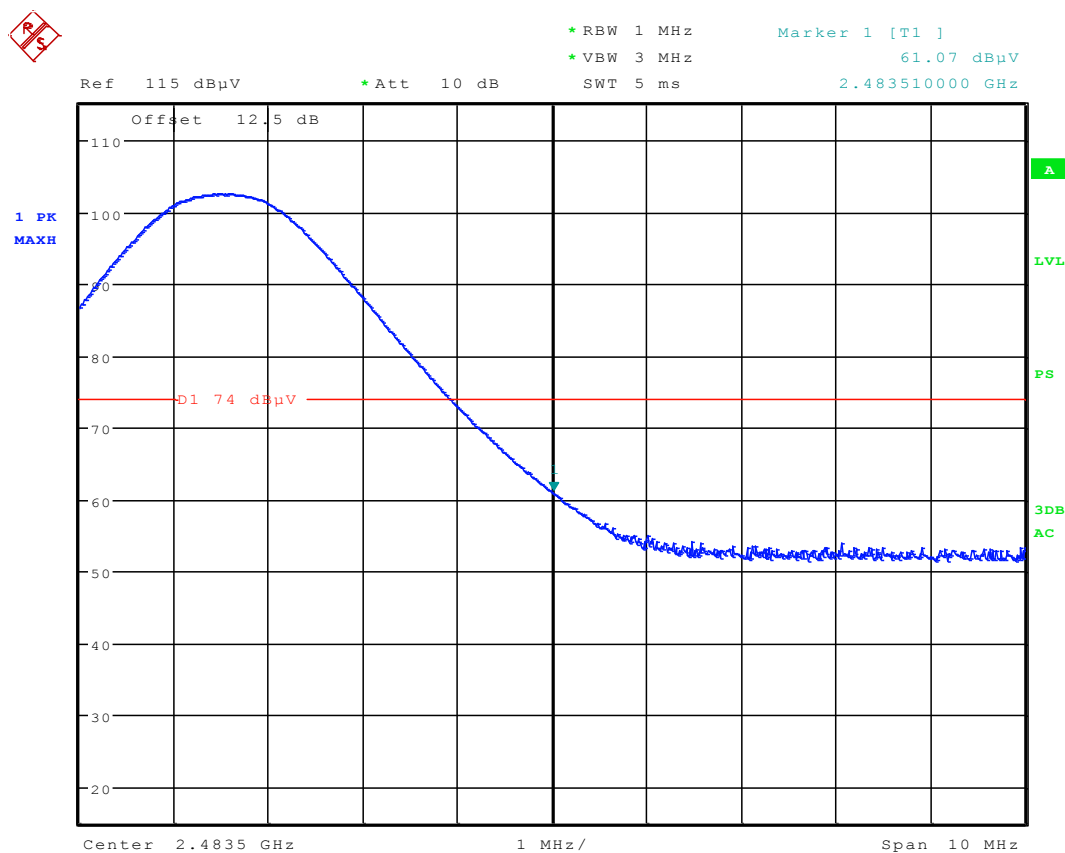
Plot 6-43. Radiated Restricted Upper Band Edge Measurement (Peak)
