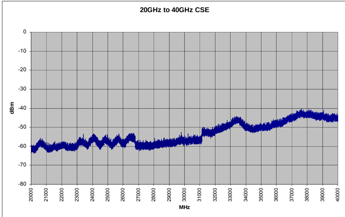
Plot 6-52. Conducted Spurious Plot (802.11a – Ch. 161)
