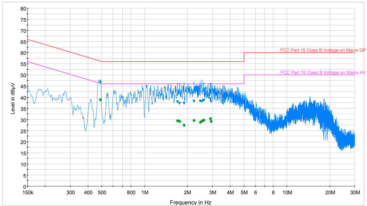
Plot 6-53. Line Conducted Plot with 802.11b (L1)
