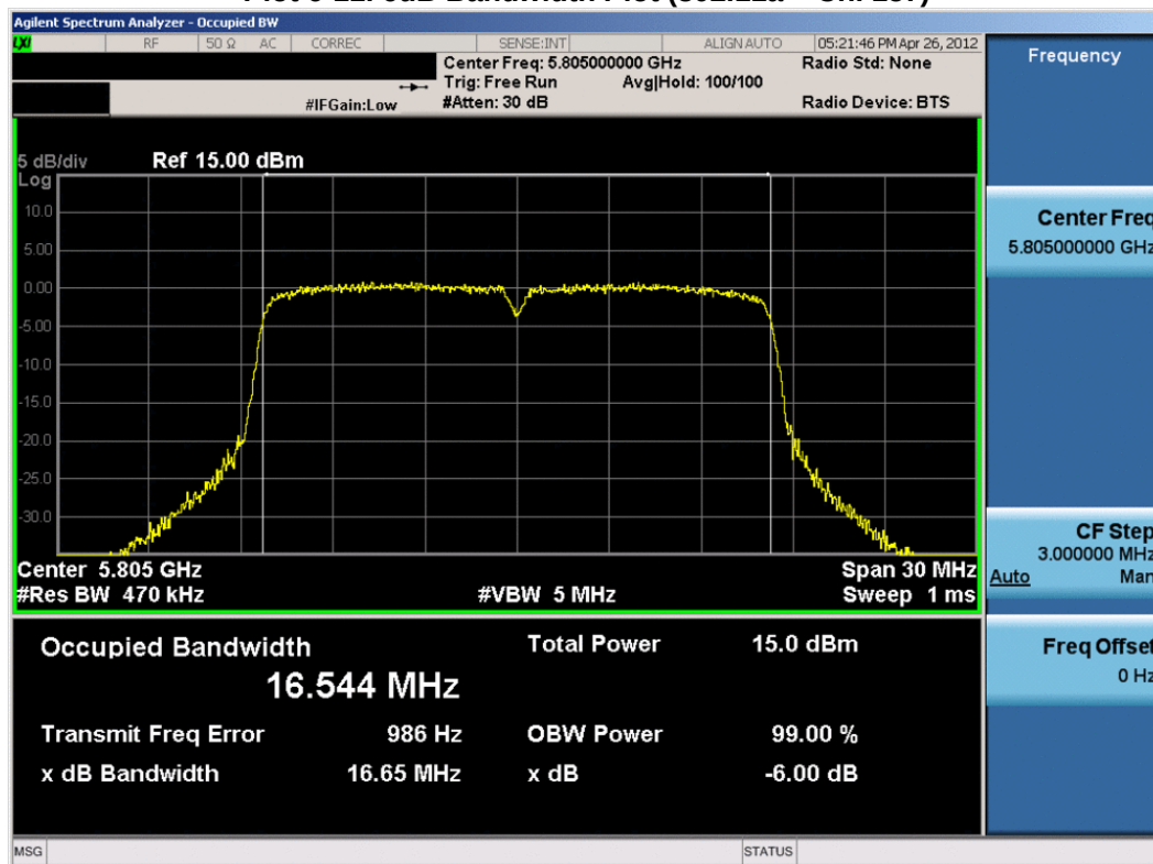
Plot 6-12. 6dB Bandwidth Plot (802.11a – Ch. 161)
