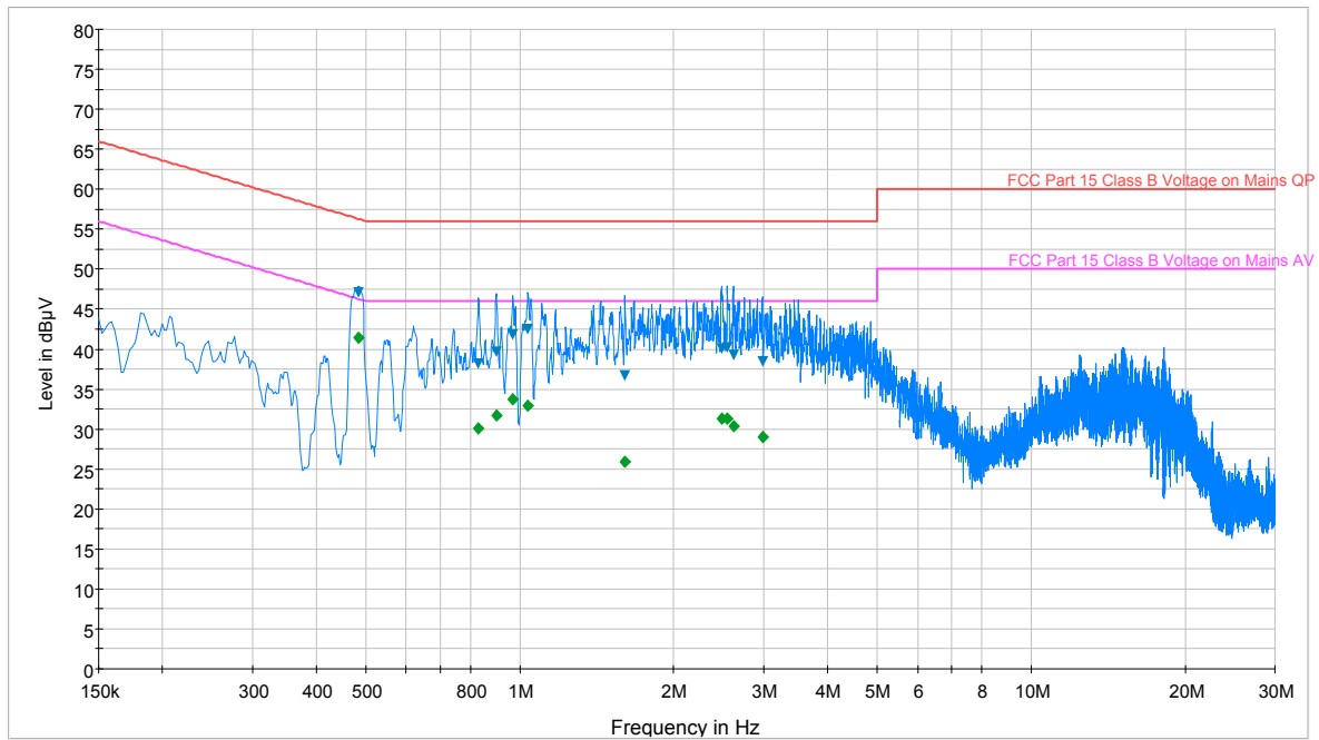
Plot 6-58. Line Conducted Plot with 802.11a (L1)
