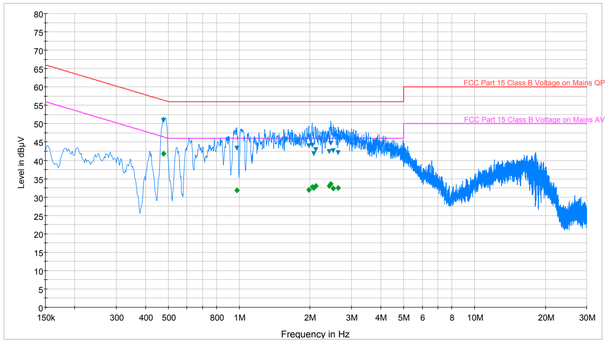
Plot 6-57. Line Conducted Plot with 802.11b (N)
