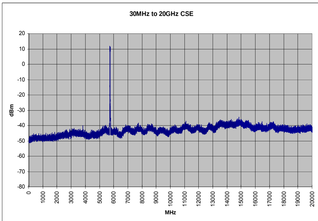
Plot 6-47. Conducted Spurious Plot (802.11a – Ch. 149)
