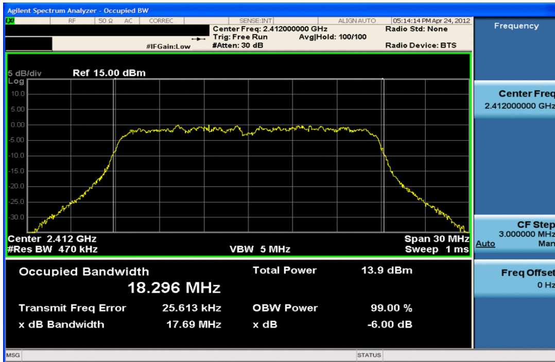
Plot 6-7. 6dB Bandwidth Plot (802.11n (2.4GHz) – Ch. 1)
