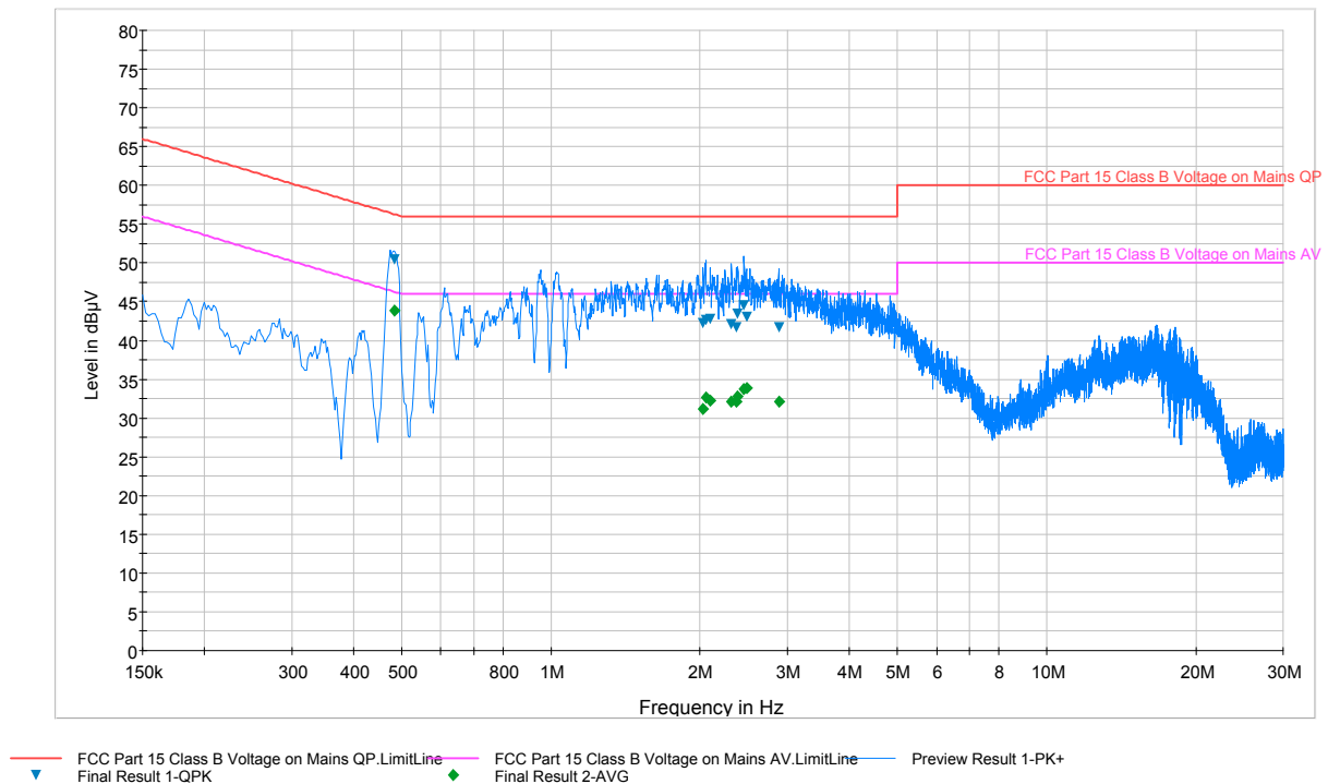
Plot 6-59. Line Conducted Plot with 802.11a (N)
