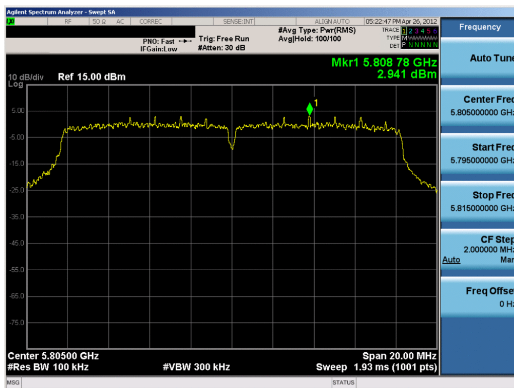
Plot 6-27. Power Spectral Density Plot (802.11a – Ch. 161)
