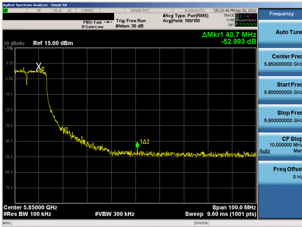
Plot 6-38. Band Edge Plot (802.11a – Ch. 161)
