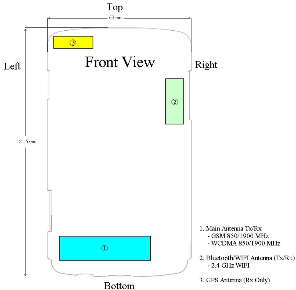
Figure 1-1 DUT Antenna Locations
