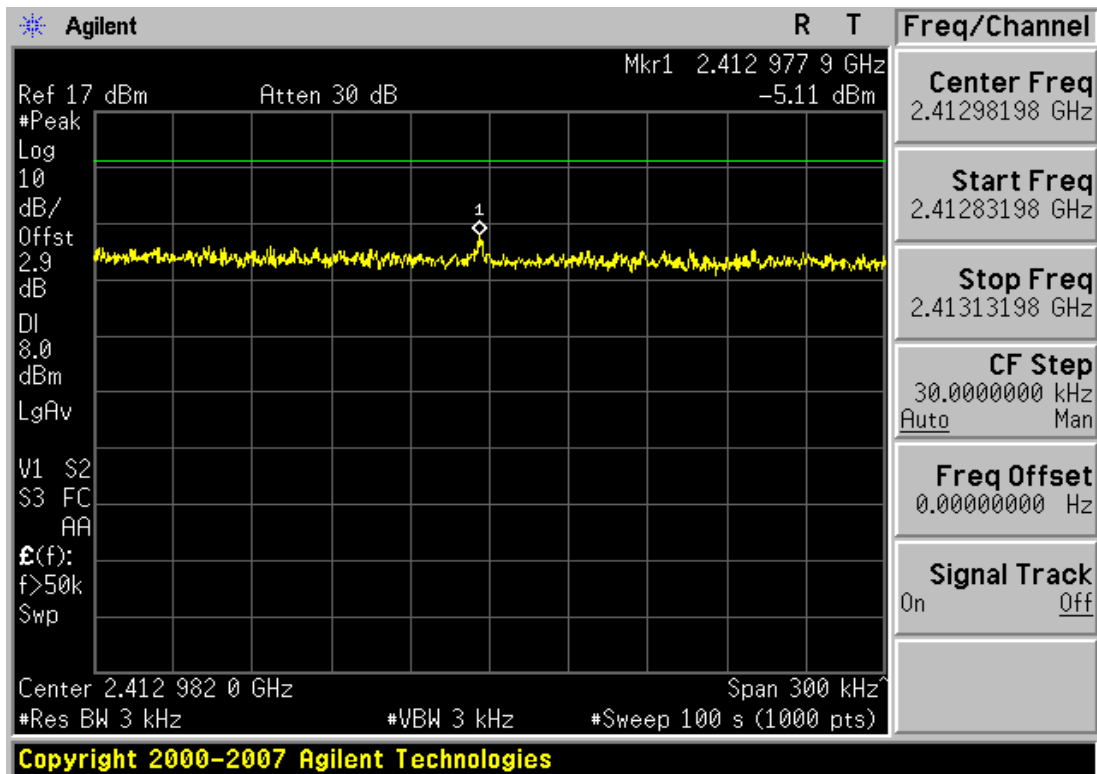
Plot 6-4. Power Spectral Density Plot (802.11b – Ch. 1)
