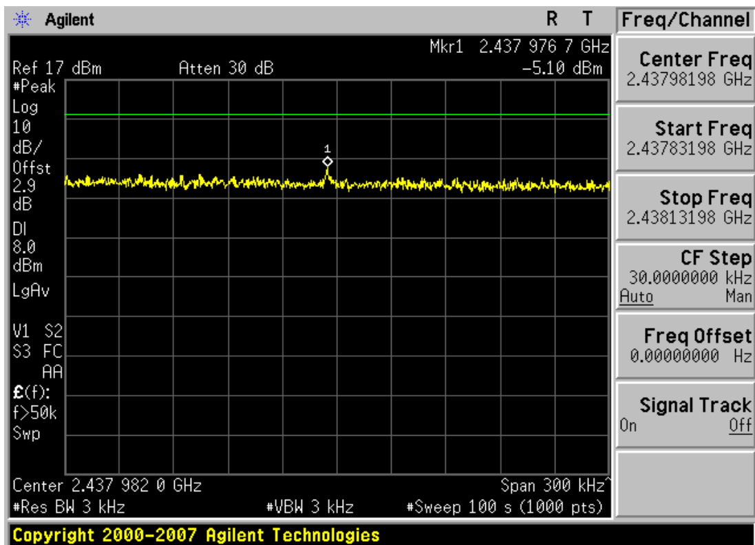
Plot 6-5. Power Spectral Density Plot (802.11b – Ch. 6)
