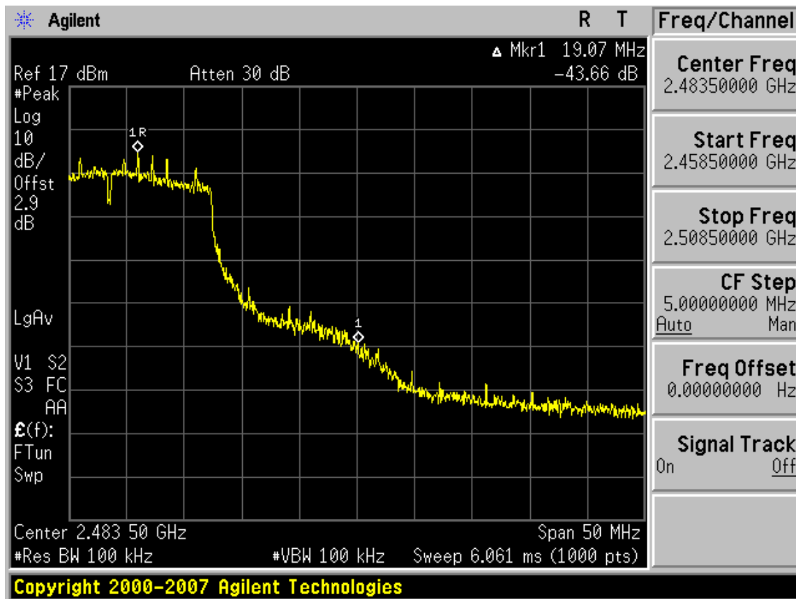
Plot 6-12. Band Edge Plot (802.11n – Ch. 11)
