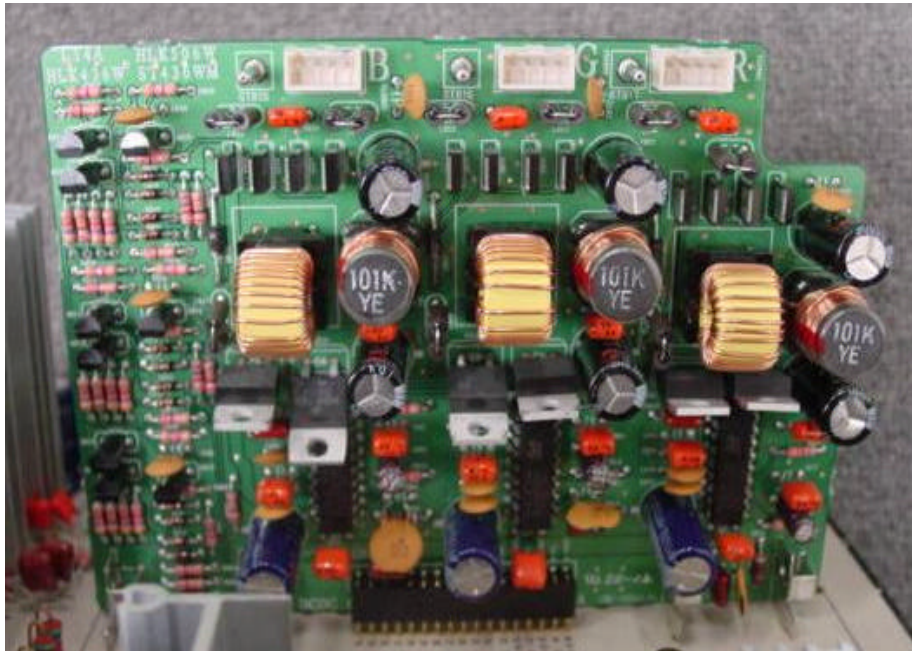
Front view of DC/DC Module PCB
