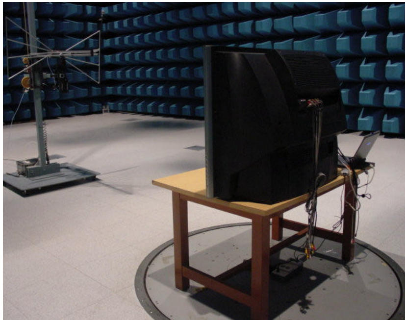
Radiated Emission (Rear view)
