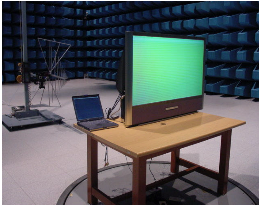
Radiated Emission (Front view)
