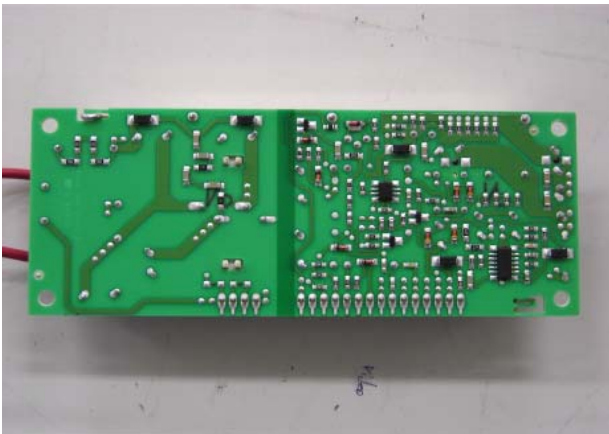
Ballast board bottom view
