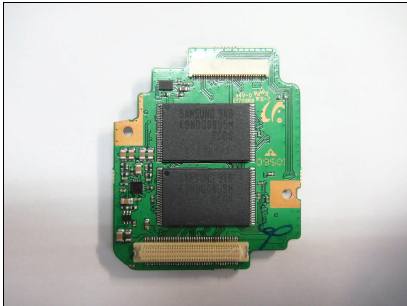
Rear view of Main PCB
