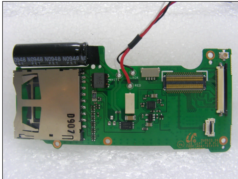
Rear view of LEFT Board
