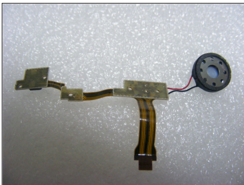
Rear view of RIGHT FPC
