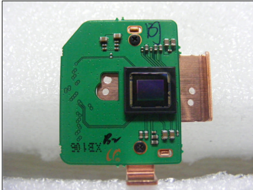
Rear view of CIS Board
