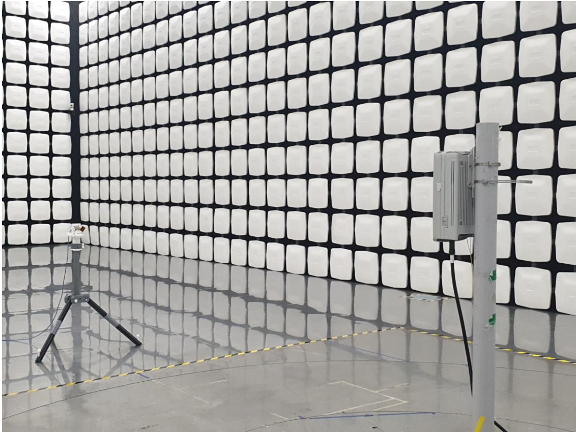
Radiated Test Setup Photo – Spurious (40 GHz ~ 60 GHz)
