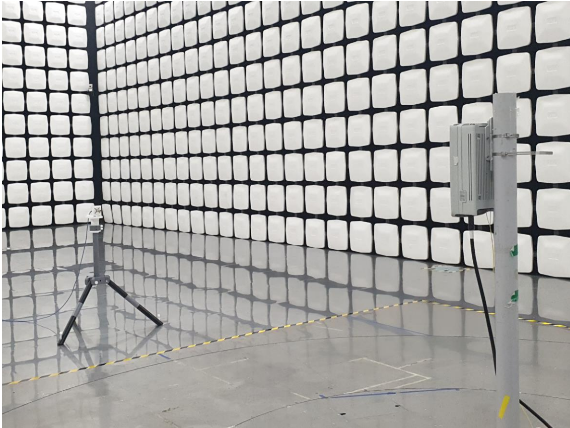
Radiated Test Setup Photo – Spurious (140 GHz ~ 200 GHz)
