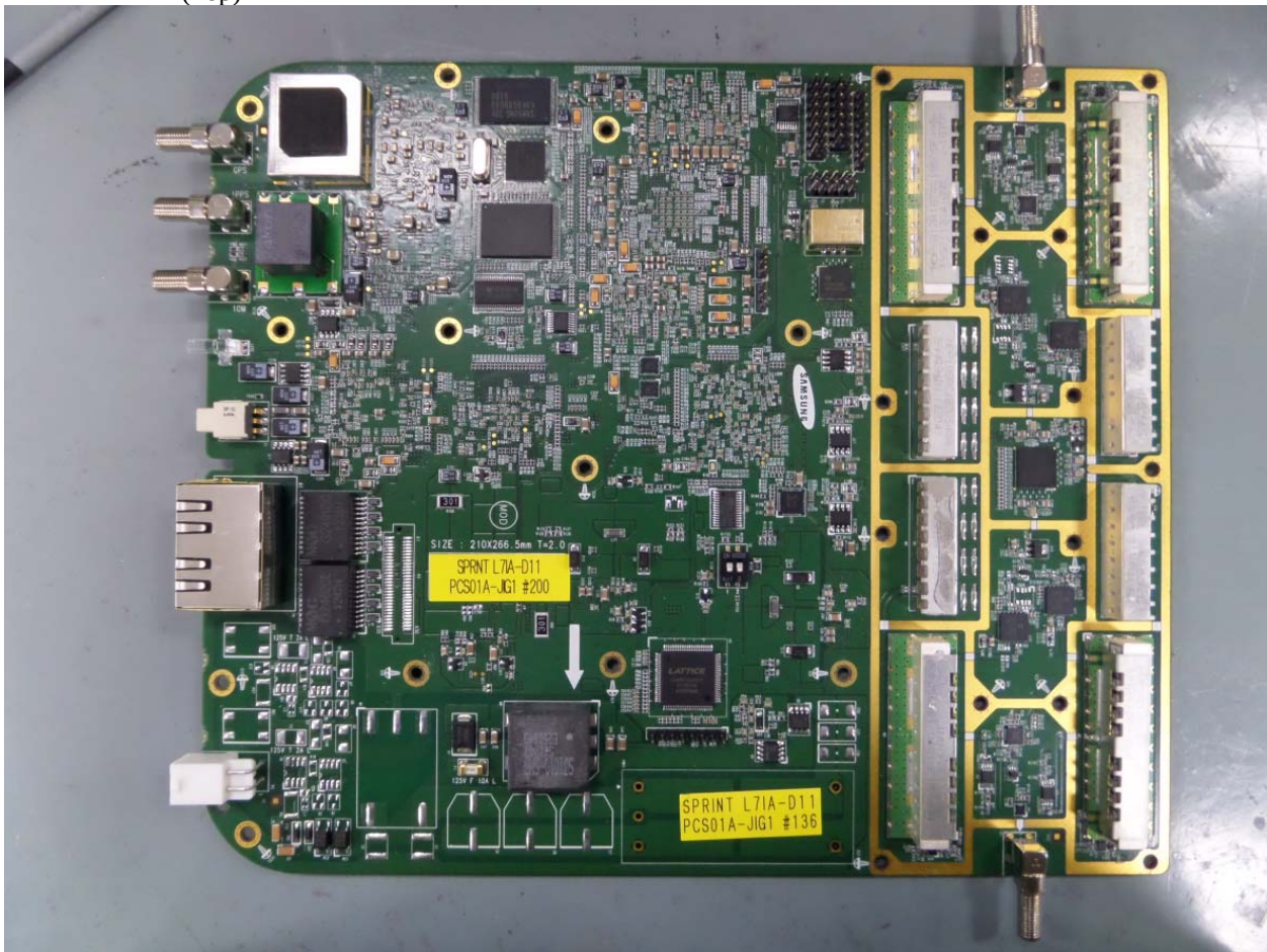
L7IA-D11 PBA (Top)
