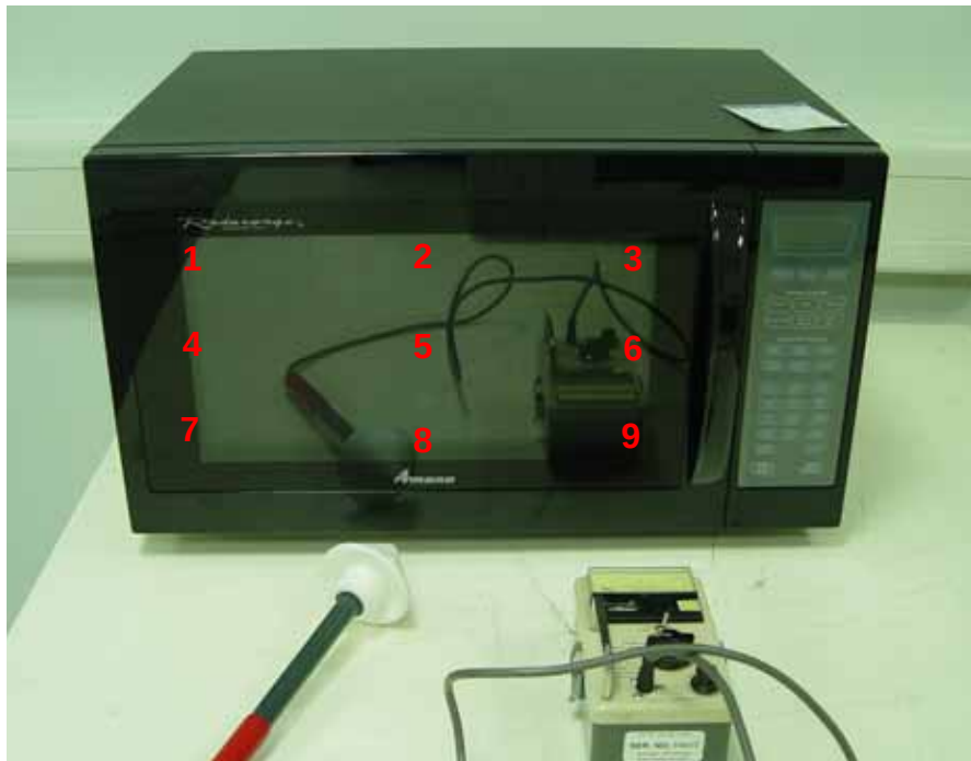
Fig. 1 Test Setup for Radiation Hazard Measurement
