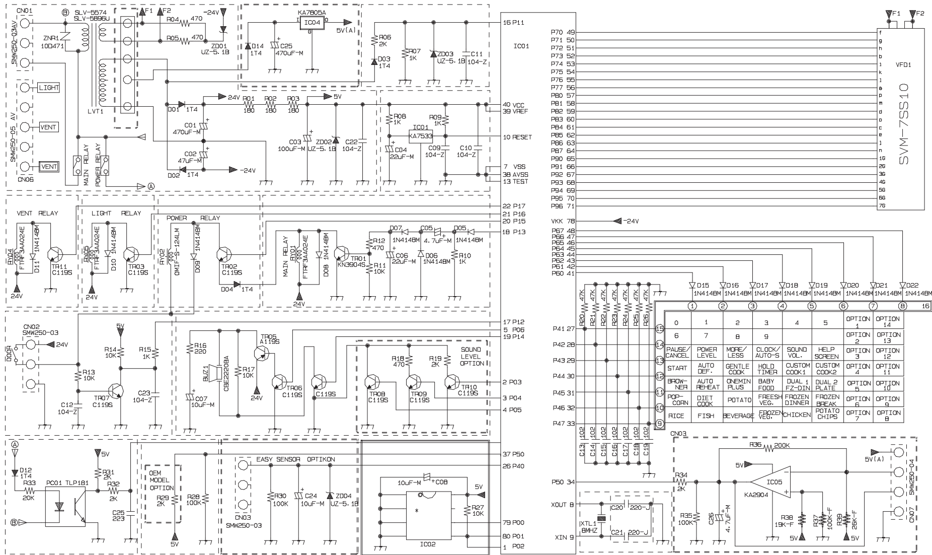
S22USA SCHEMATIC
