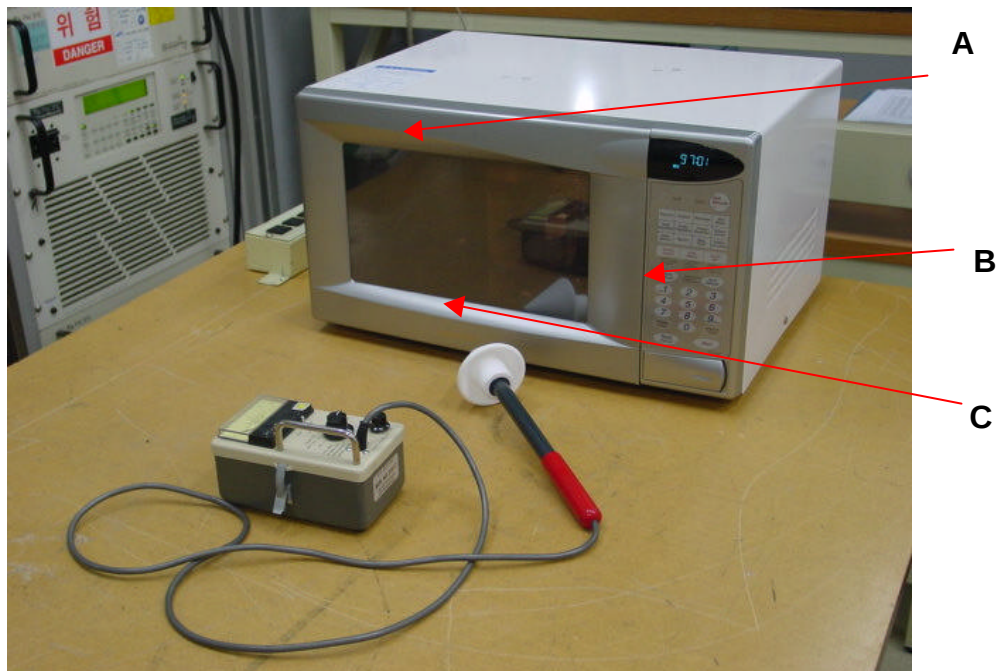
Fig. 1 Test Setup and the locations of maximum leakage
