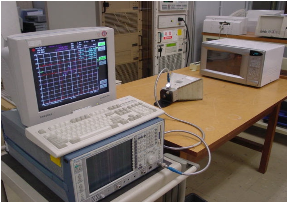
Fig. 5 Test Setup for Operating Frequency Measurements
