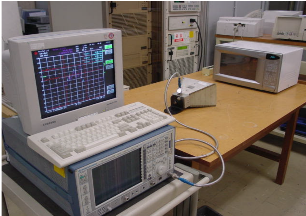
Fig. 2 Test Setup for Input power
