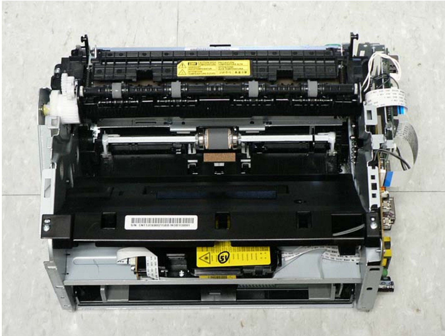
ML-1670_Internal_Top Side
