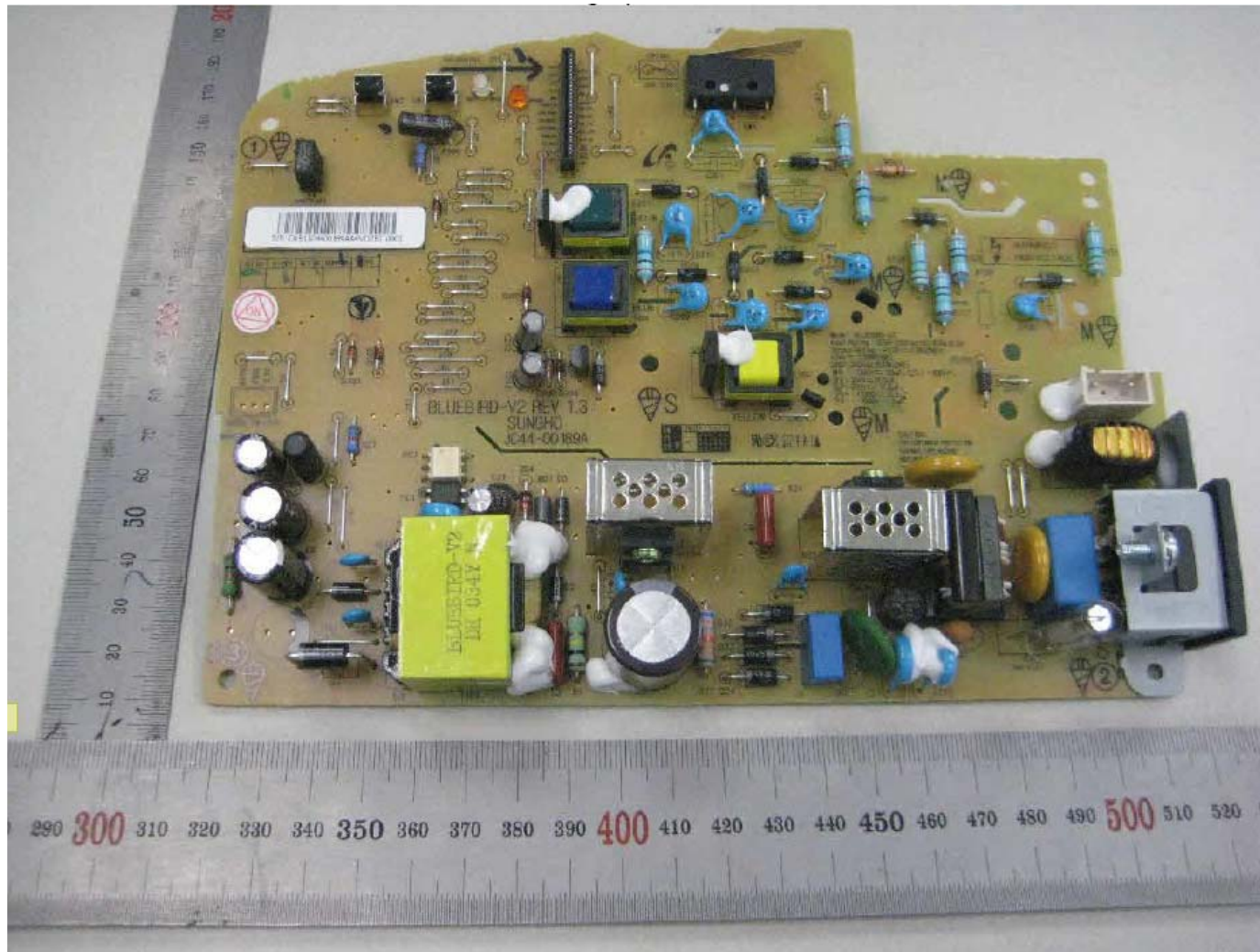
SUNGHO, Bluebird_V2 (ML-1670_SMPS PBA_Top Side)
