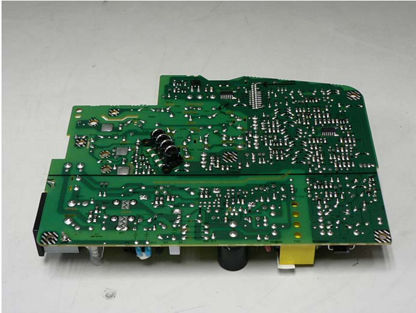
신강위(SHANDONG COWI), Bluebird_V2 (ML-1670_SMPS PBA_TOP Side)
