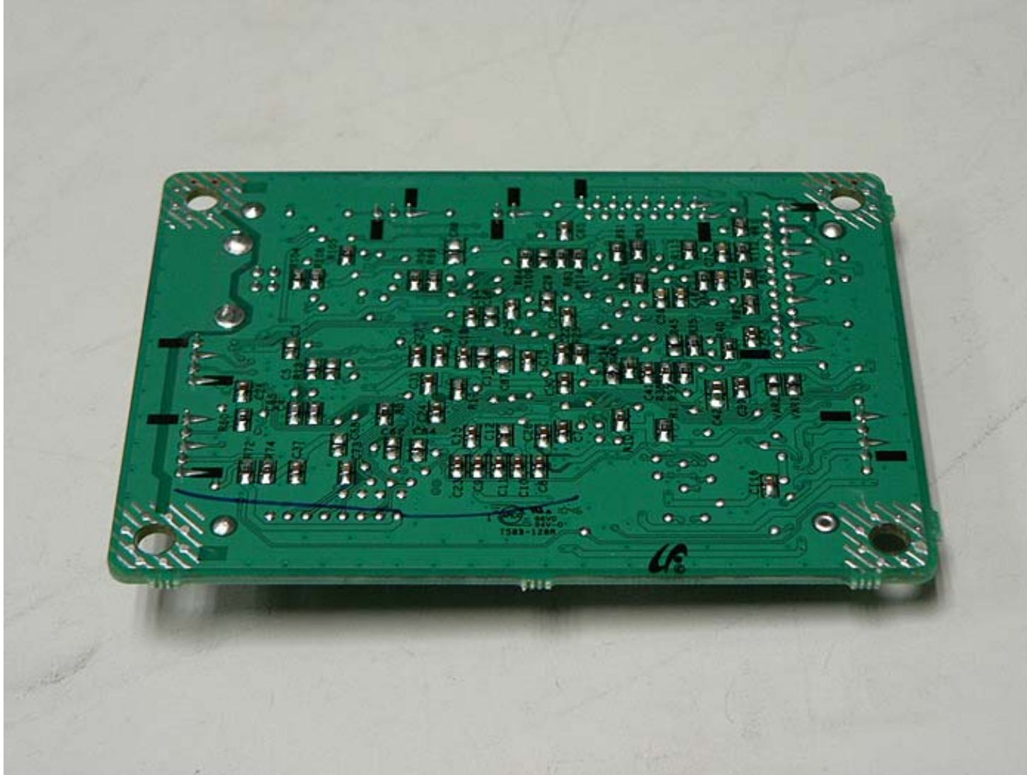
ML-1670_Main PBA_Bottom side
