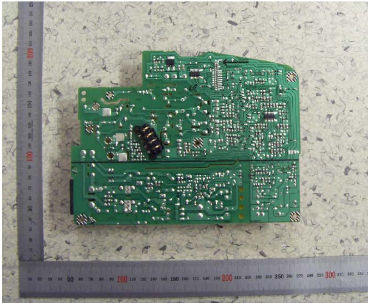
SCTH, Bluebird_V2 (ML-1670_SMPS PBA_Bottom Side)
