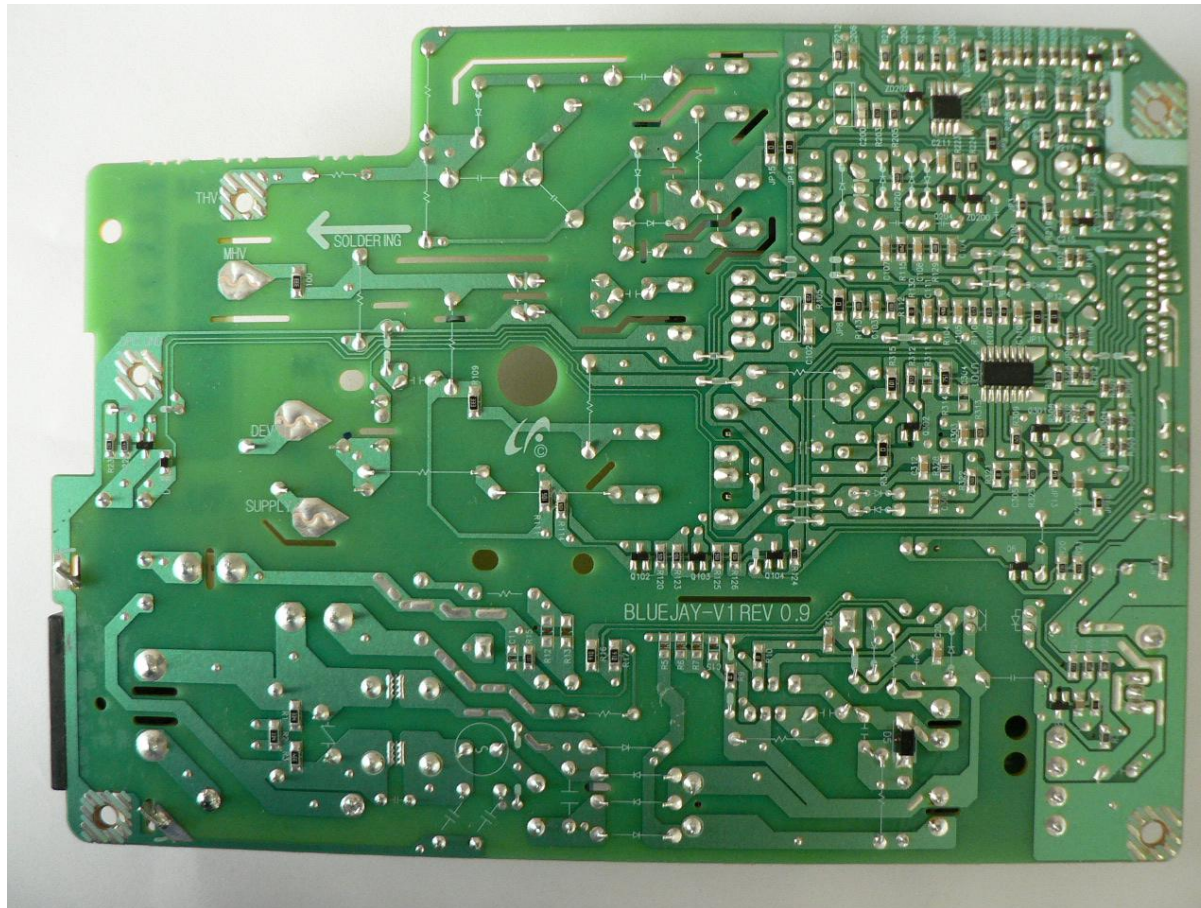
SUNGHO, Bluejay V1 ML-2164 SMPS & HVPS PBA_Rear
