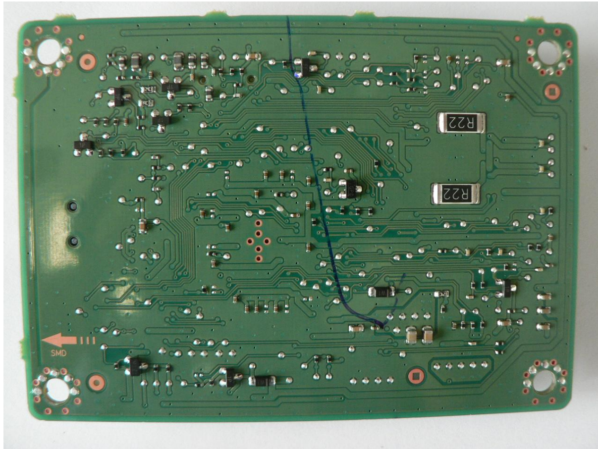
ML-2164 Main PBA_Bottom
