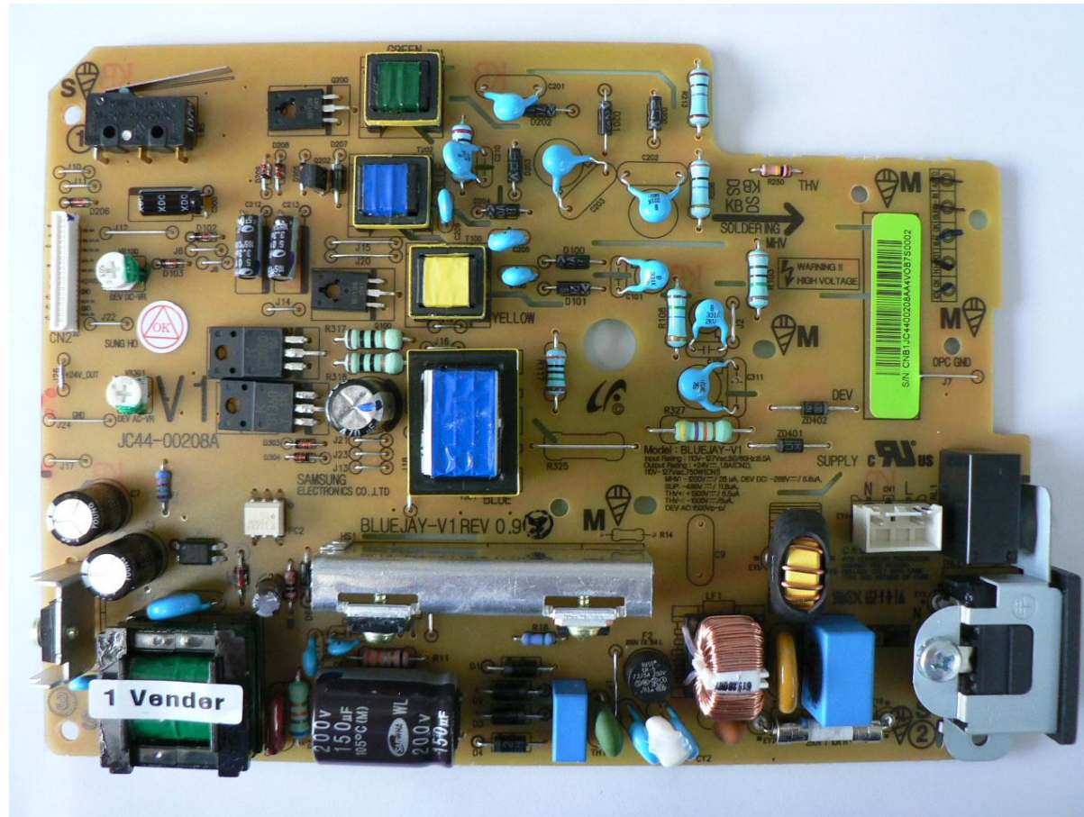
SUNGHO, Bluejay V1 ML-2164 SMPS & HVPS PBA_Front
