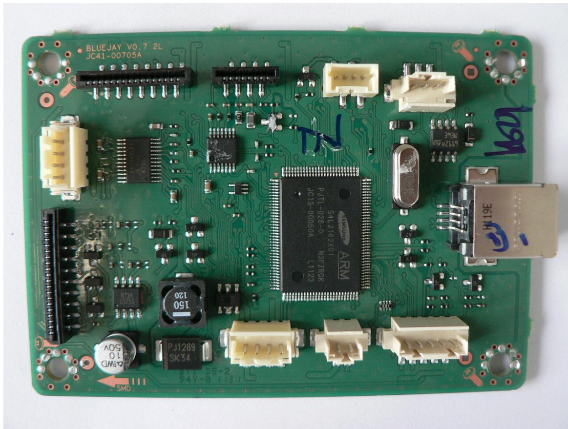
ML-2164 Main PBA_Top
