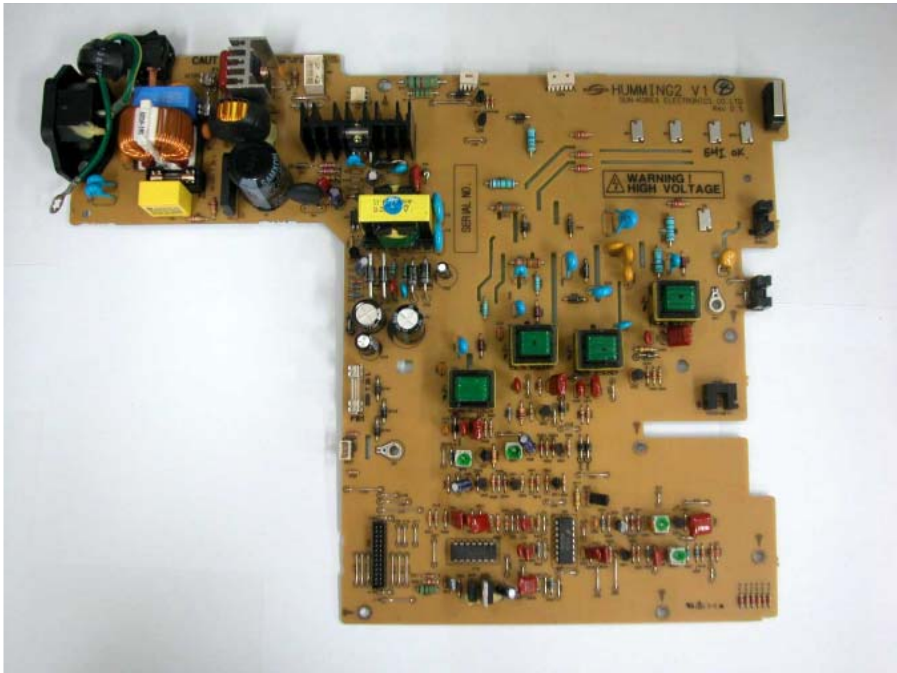
Top View of SMPS + HVPS
