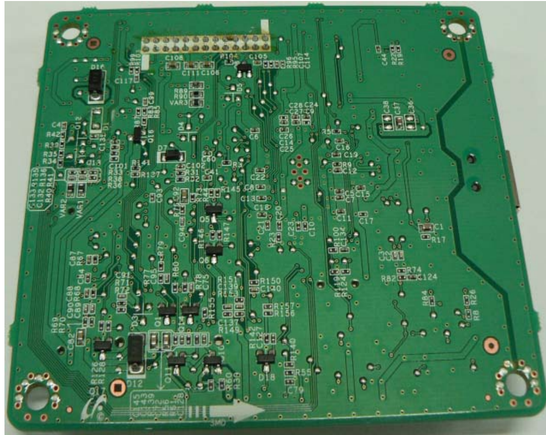
ML-2540 Main PBA_Rear
