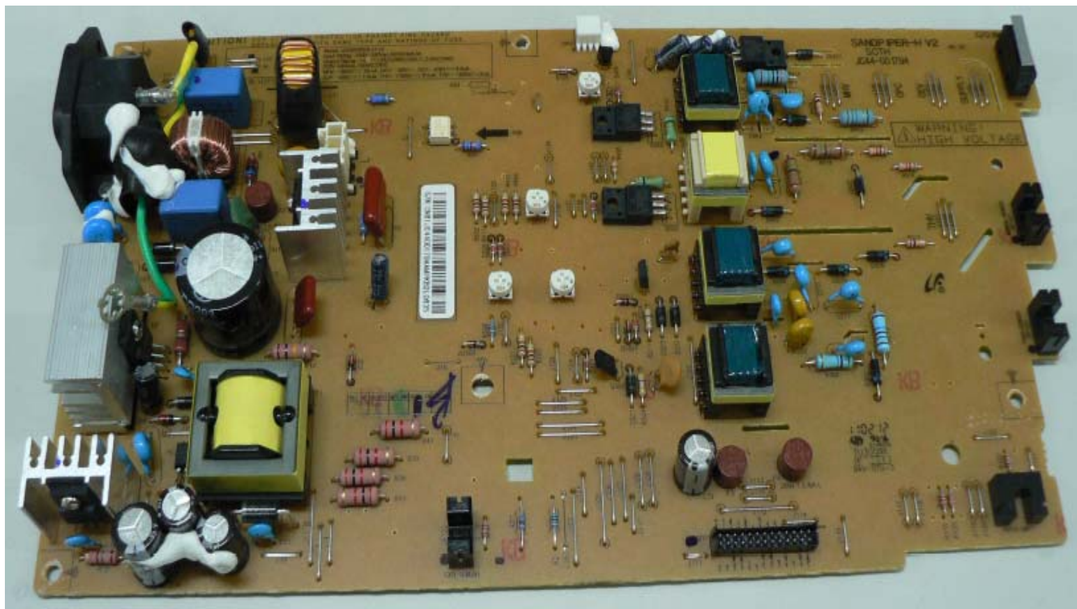
SCTH , SANDPIPER-H V2 ML-2540 SMPS & HVPS PBA_Front
