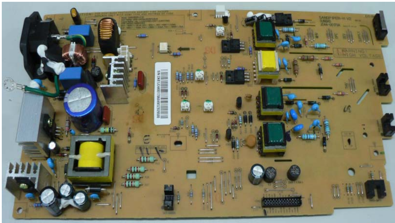
SUNGHO , SANDPIPER-H V2 ML-2540 SMPS & HVPS PBA_Front
