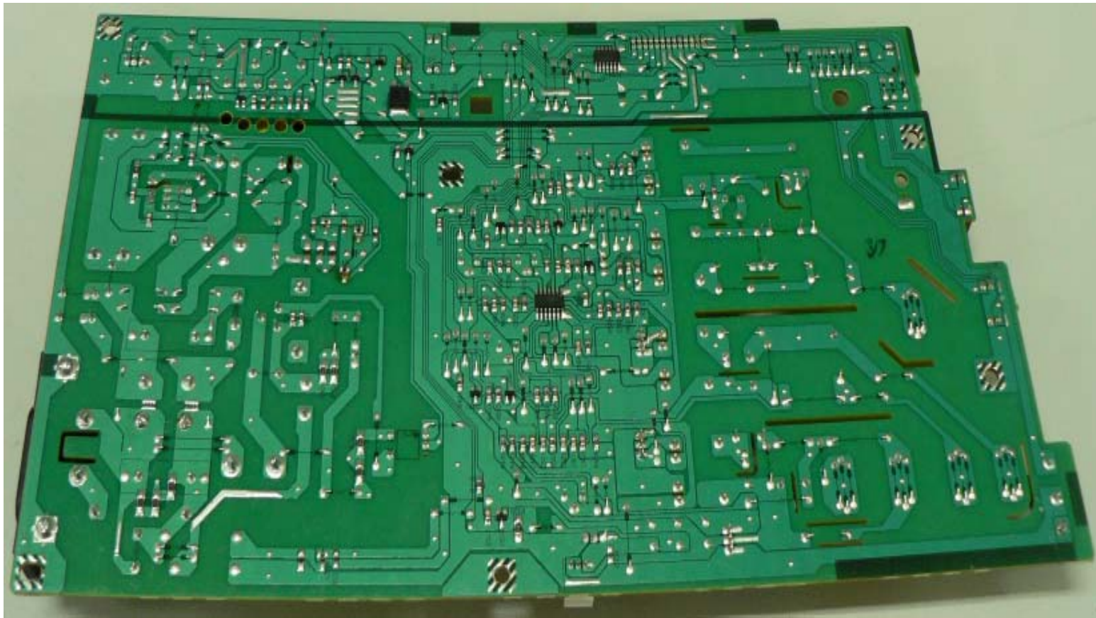
SUNGHO , SANDPIPER-H V2 ML-2540 SMPS & HVPS PBA_Rear
