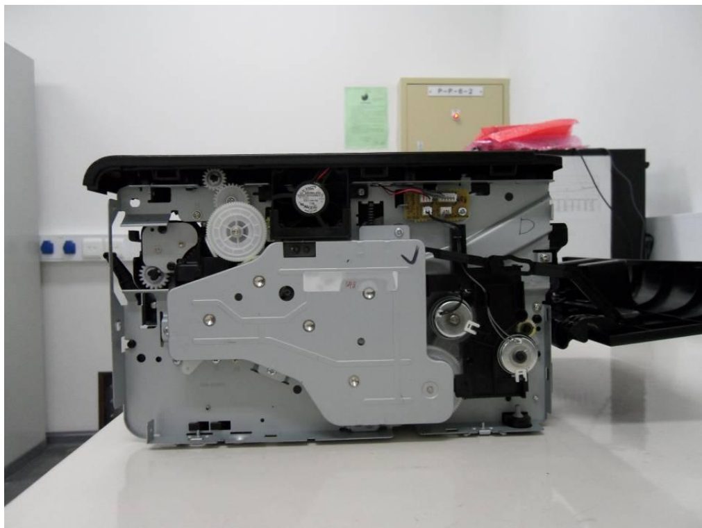
Internal View(left)
