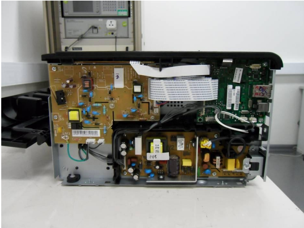
Internal View(right)
