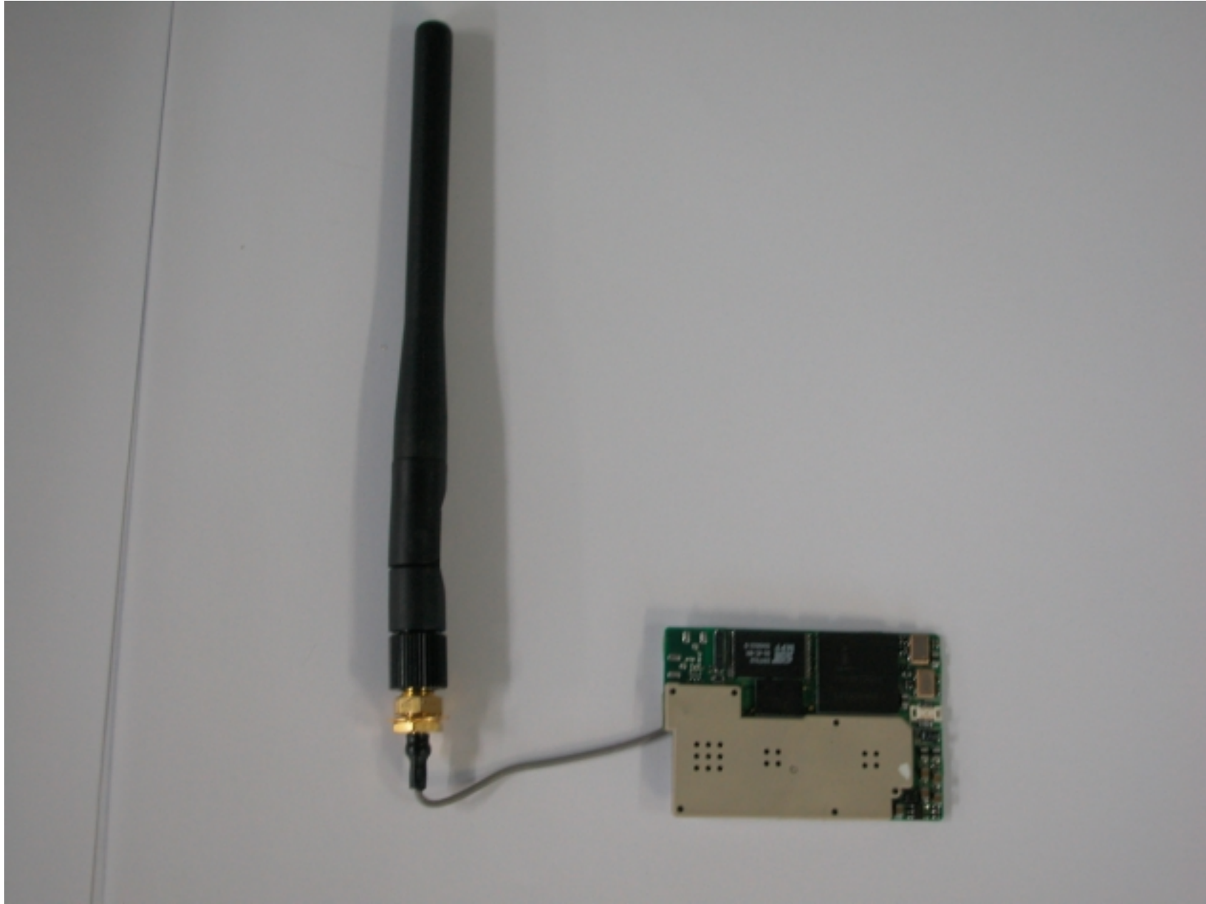
Top View of WLAN module
