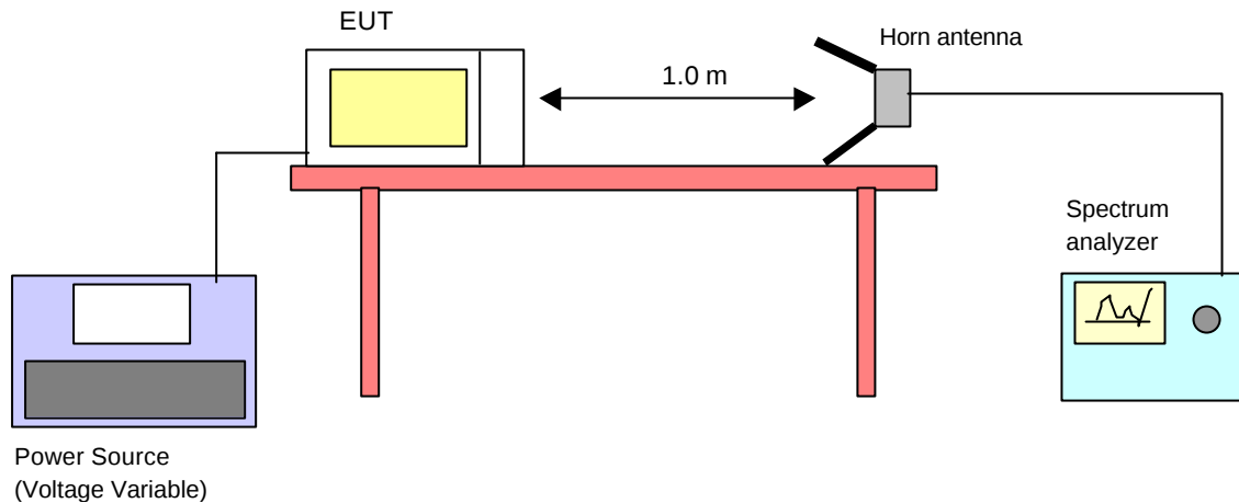
Fig. 2 Operating Frequency Measurements Configuration
